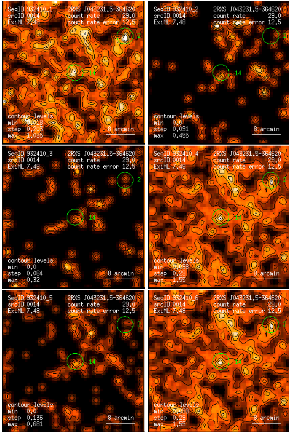
Figure 14: RASS 932410: detection 0014: band rate images, Gaussian filter: (1) PSPC channels 11 – 41, (2) 52 – 90, (3) 91 – 201, (4) 11 – 235, (5) 52 – 201, (6) 11 – 201. Broad band rates in counts/ks. Band rate contour levels in counts/ks/arcmin 2 .
