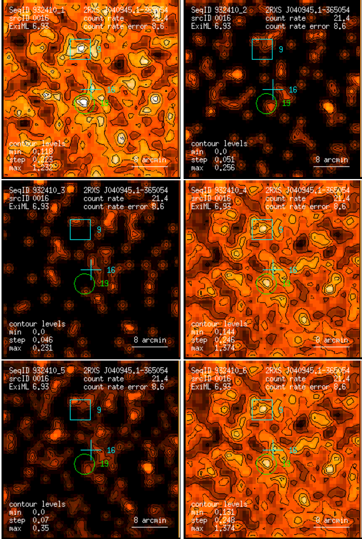
Figure 16: RASS 932410: detection 0016: band rate images, Gaussian filter: (1) PSPC channels 11 – 41, (2) 52 – 90, (3) 91 – 201, (4) 11 – 235, (5) 52 – 201, (6) 11 – 201. Broad band rates in counts/ks. Band rate contour levels in counts/ks/arcmin 2 .
