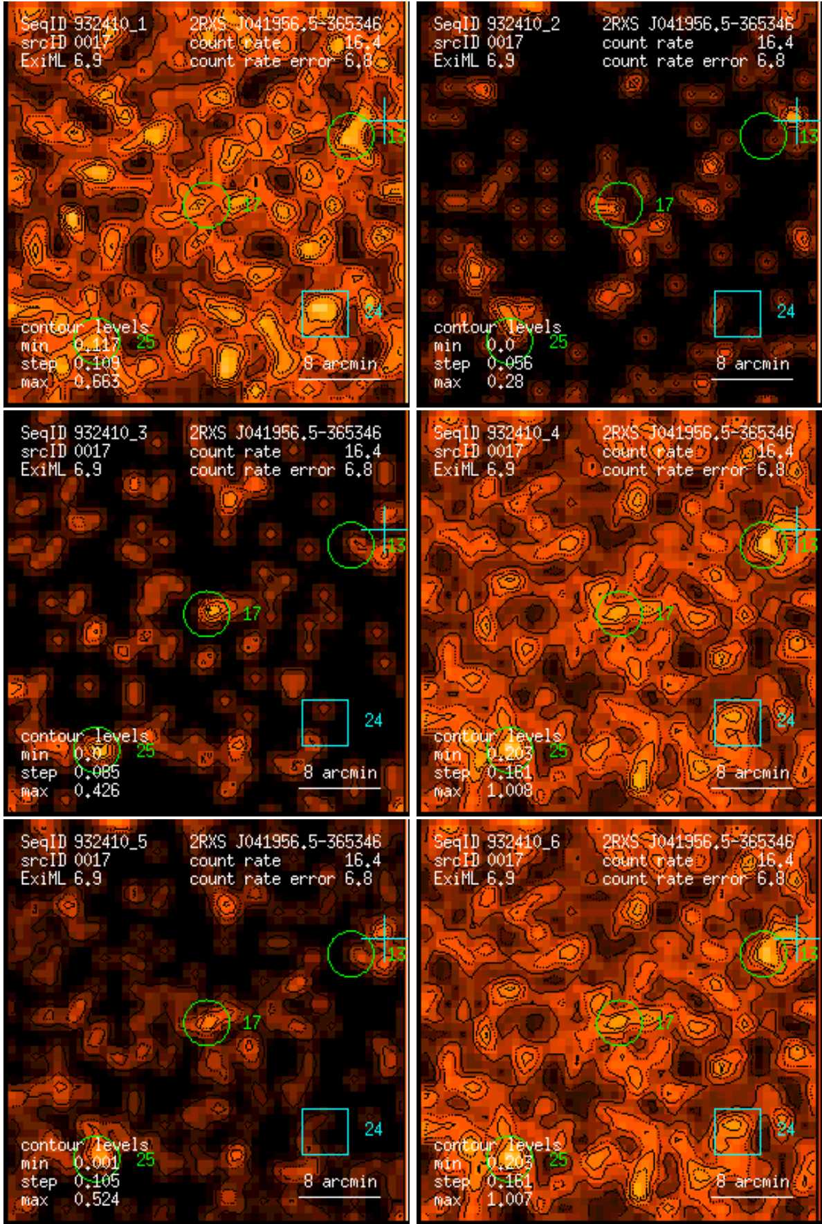
Figure 17: RASS 932410: detection 0017: band rate images, Gaussian filter: (1) PSPC channels 11 – 41, (2) 52 – 90, (3) 91 – 201, (4) 11 – 235, (5) 52 – 201, (6) 11 – 201. Broad band rates in counts/ks. Band rate contour levels in counts/ks/arcmin 2 .
