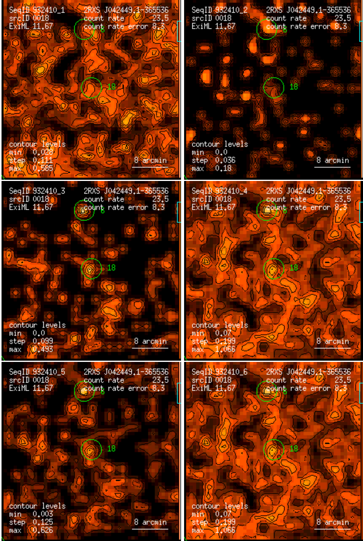
Figure 18: RASS 932410: detection 0018: band rate images, Gaussian filter: (1) PSPC channels 11 – 41, (2) 52 – 90, (3) 91 – 201, (4) 11 – 235, (5) 52 – 201, (6) 11 – 201. Broad band rates in counts/ks. Band rate contour levels in counts/ks/arcmin 2 .
