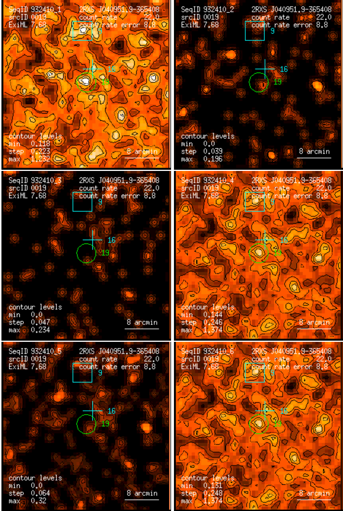
Figure 19: RASS 932410: detection 0019: band rate images, Gaussian filter: (1) PSPC channels 11 – 41, (2) 52 – 90, (3) 91 – 201, (4) 11 – 235, (5) 52 – 201, (6) 11 – 201. Broad band rates in counts/ks. Band rate contour levels in counts/ks/arcmin 2 .
