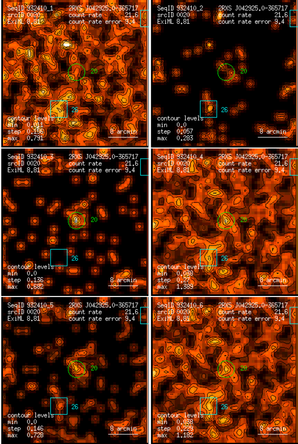
Figure 20: RASS 932410: detection 0020: band rate images, Gaussian filter: (1) PSPC channels 11 – 41, (2) 52 – 90, (3) 91 – 201, (4) 11 – 235, (5) 52 – 201, (6) 11 – 201. Broad band rates in counts/ks. Band rate contour levels in counts/ks/arcmin 2 .
