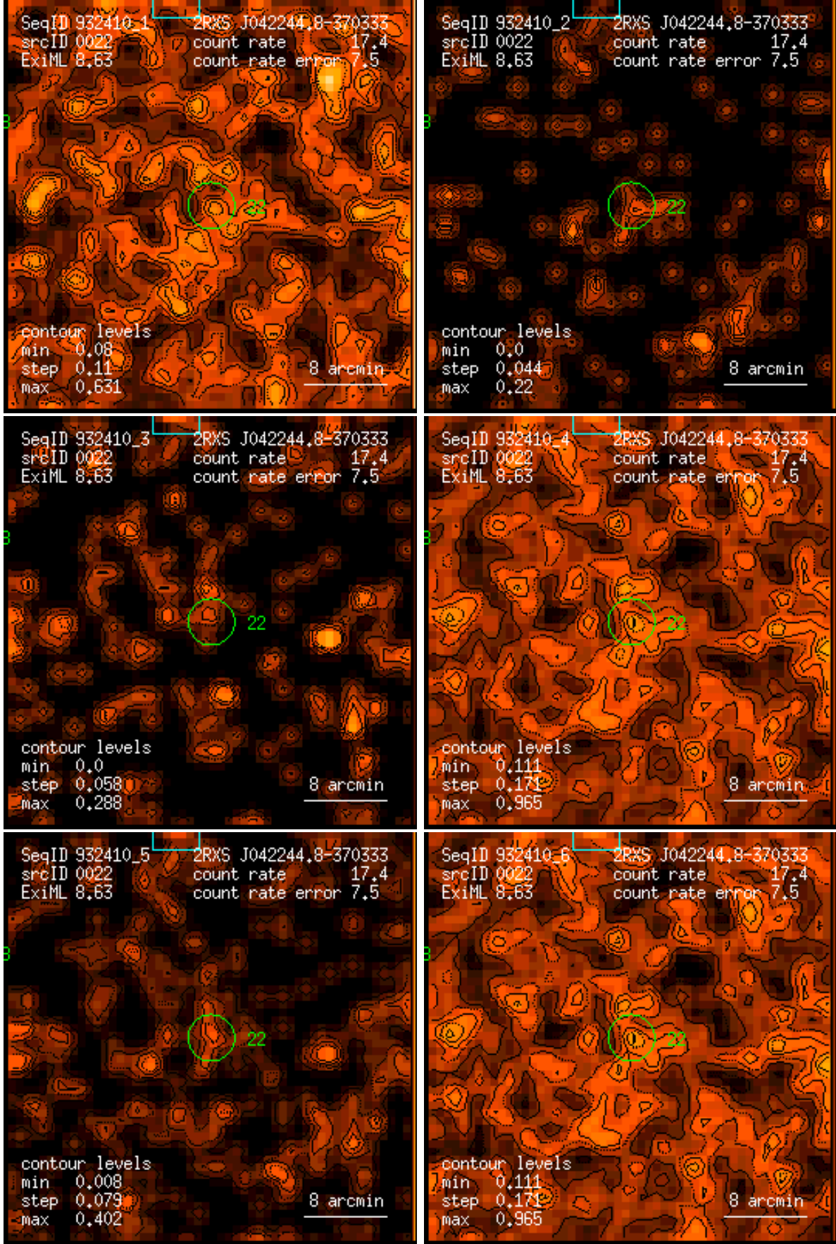
Figure 22: RASS 932410: detection 0022: band rate images, Gaussian filter: (1) PSPC channels 11 – 41, (2) 52 – 90, (3) 91 – 201, (4) 11 – 235, (5) 52 – 201, (6) 11 – 201. Broad band rates in counts/ks. Band rate contour levels in counts/ks/arcmin 2 .
