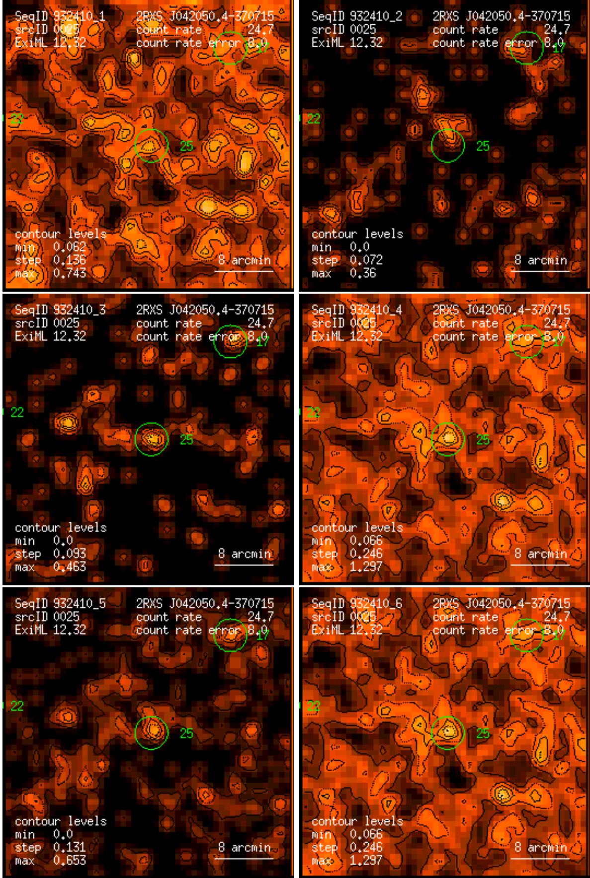
Figure 25: RASS 932410: detection 0025: band rate images, Gaussian filter: (1) PSPC channels 11 – 41, (2) 52 – 90, (3) 91 – 201, (4) 11 – 235, (5) 52 – 201, (6) 11 – 201. Broad band rates in counts/ks. Band rate contour levels in counts/ks/arcmin 2 .
