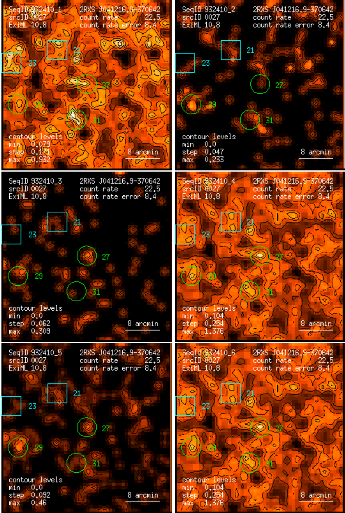
Figure 27: RASS 932410: detection 0027: band rate images, Gaussian filter: (1) PSPC channels 11 – 41, (2) 52 – 90, (3) 91 – 201, (4) 11 – 235, (5) 52 – 201, (6) 11 – 201. Broad band rates in counts/ks. Band rate contour levels in counts/ks/arcmin 2 .
