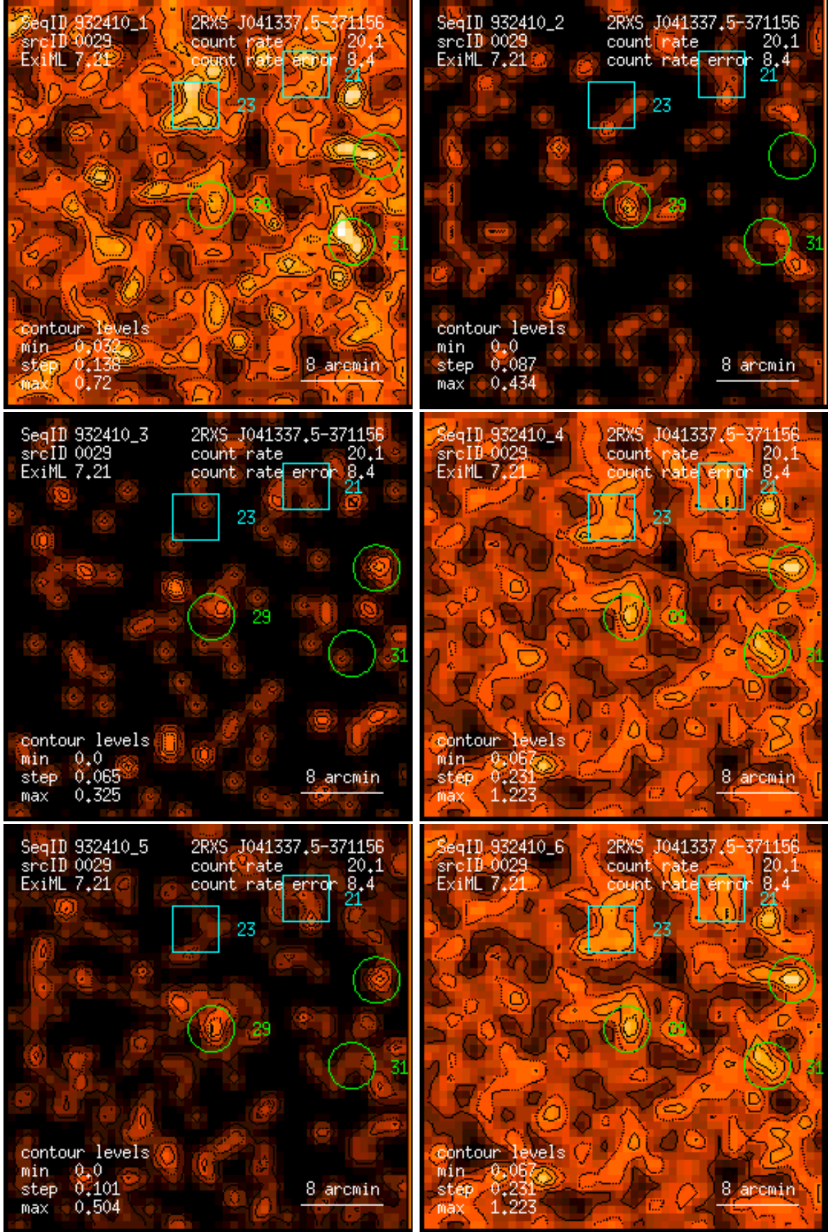
Figure 29: RASS 932410: detection 0029: band rate images, Gaussian filter: (1) PSPC channels 11 – 41, (2) 52 – 90, (3) 91 – 201, (4) 11 – 235, (5) 52 – 201, (6) 11 – 201. Broad band rates in counts/ks. Band rate contour levels in counts/ks/arcmin 2 .
