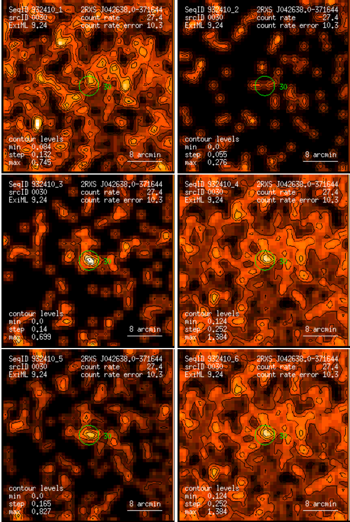
Figure 30: RASS 932410: detection 0030: band rate images, Gaussian filter: (1) PSPC channels 11 – 41, (2) 52 – 90, (3) 91 – 201, (4) 11 – 235, (5) 52 – 201, (6) 11 – 201. Broad band rates in counts/ks. Band rate contour levels in counts/ks/arcmin 2 .
