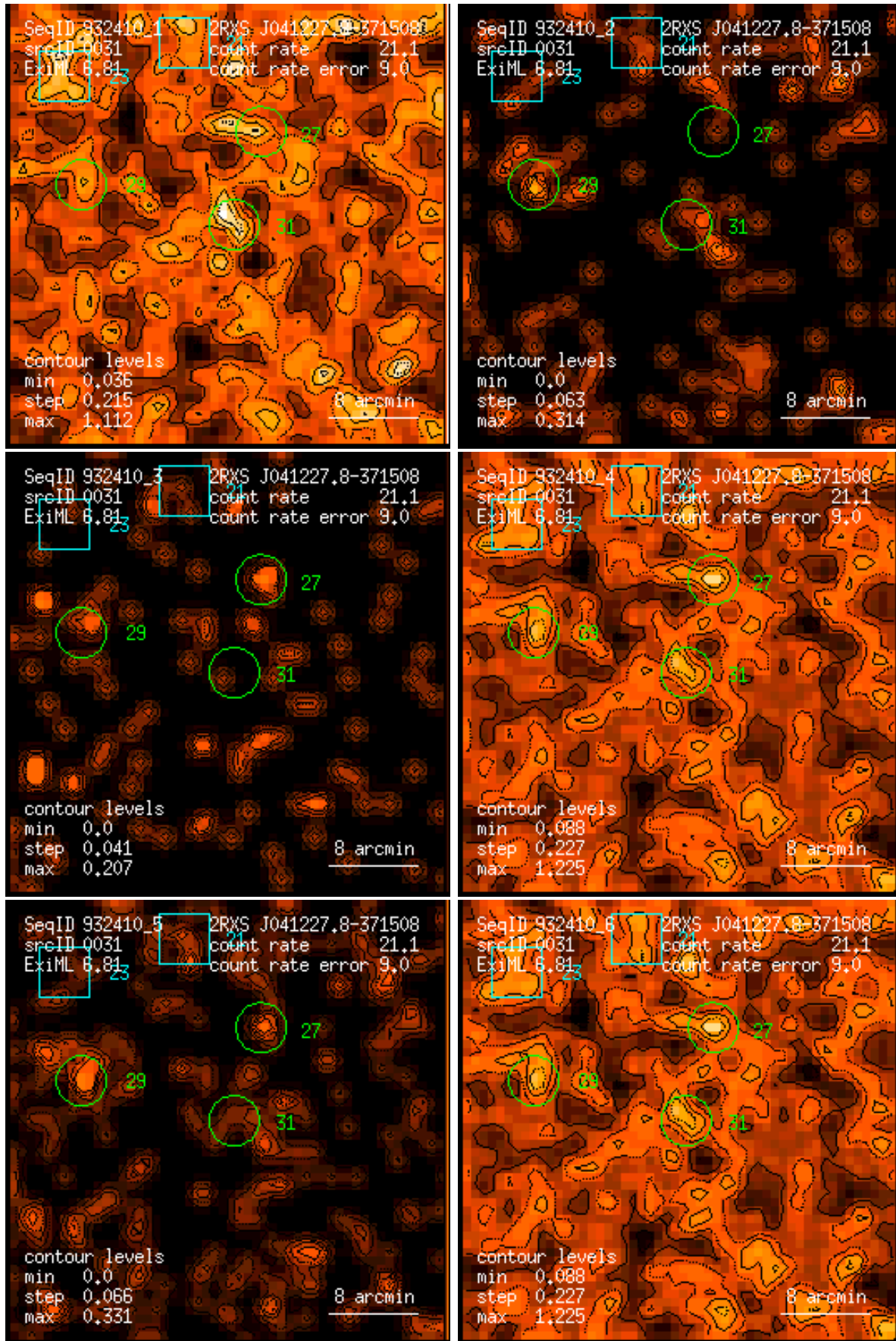
Figure 31: RASS 932410: detection 0031: band rate images, Gaussian filter: (1) PSPC channels 11 – 41, (2) 52 – 90, (3) 91 – 201, (4) 11 – 235, (5) 52 – 201, (6) 11 – 201. Broad band rates in counts/ks. Band rate contour levels in counts/ks/arcmin 2 .
