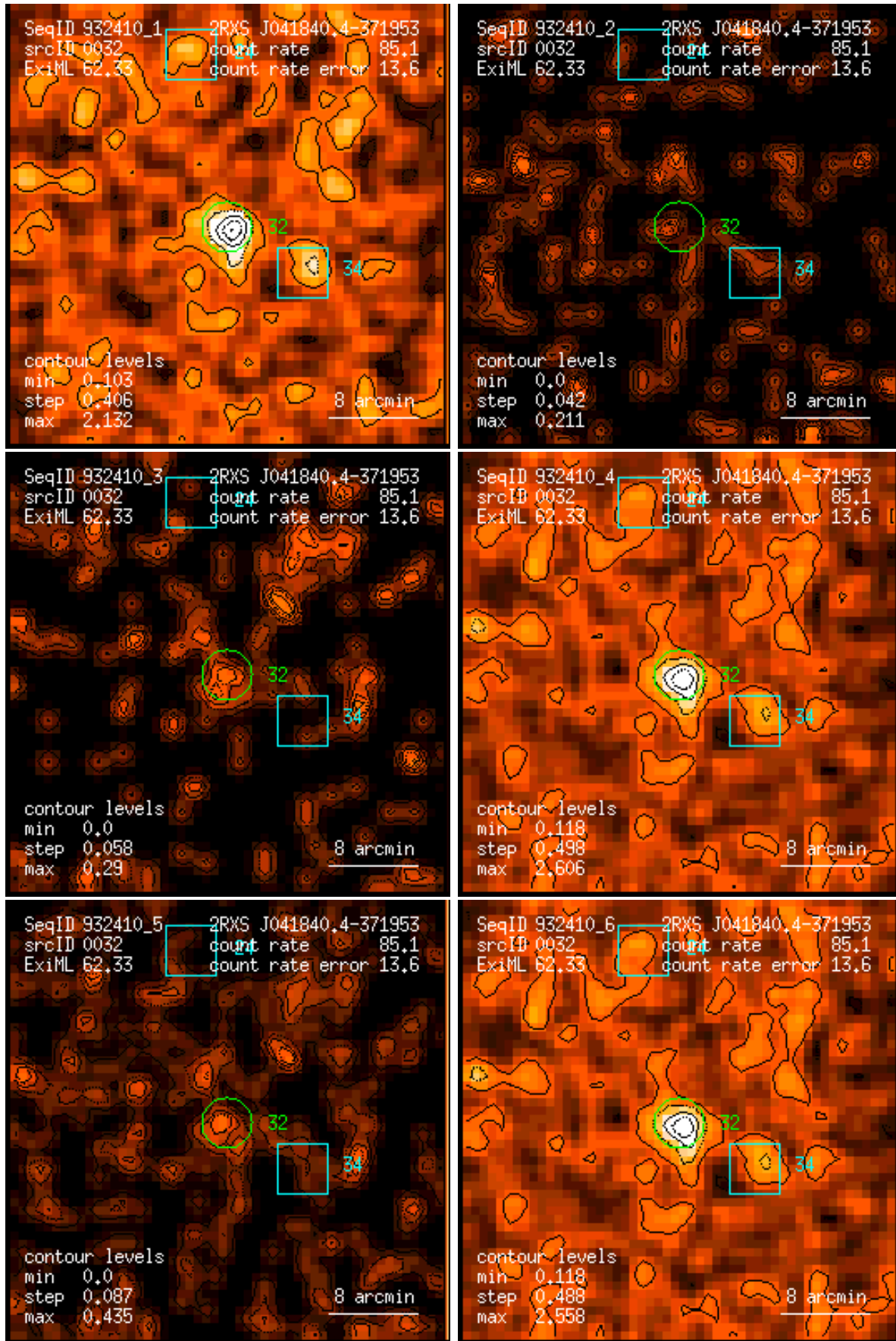
Figure 32: RASS 932410: detection 0032: band rate images, Gaussian filter: (1) PSPC channels 11 – 41, (2) 52 – 90, (3) 91 – 201, (4) 11 – 235, (5) 52 – 201, (6) 11 – 201. Broad band rates in counts/ks. Band rate contour levels in counts/ks/arcmin 2 .
