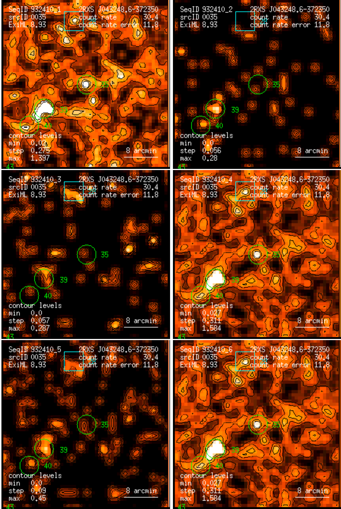
Figure 35: RASS 932410: detection 0035: band rate images, Gaussian filter: (1) PSPC channels 11 – 41, (2) 52 – 90, (3) 91 – 201, (4) 11 – 235, (5) 52 – 201, (6) 11 – 201. Broad band rates in counts/ks. Band rate contour levels in counts/ks/arcmin 2 .
