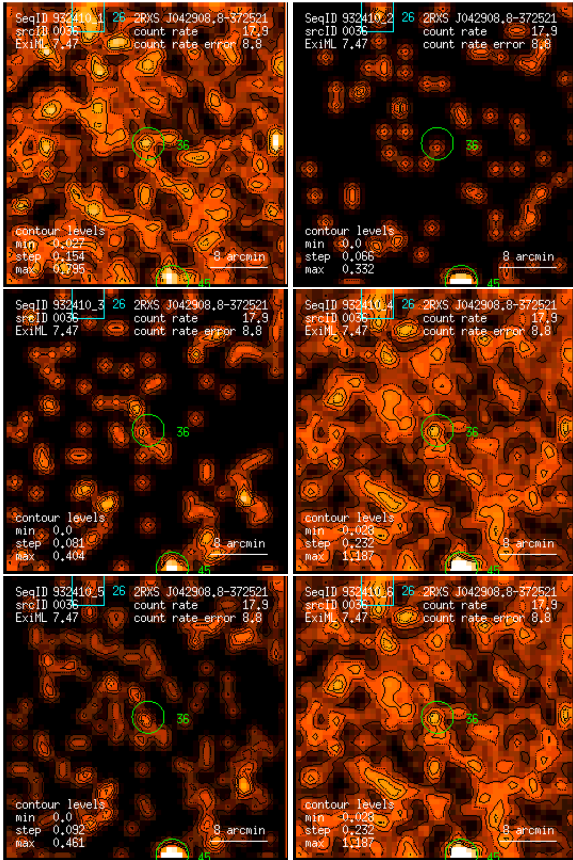
Figure 36: RASS 932410: detection 0036: band rate images, Gaussian filter: (1) PSPC channels 11 – 41, (2) 52 – 90, (3) 91 – 201, (4) 11 – 235, (5) 52 – 201, (6) 11 – 201. Broad band rates in counts/ks. Band rate contour levels in counts/ks/arcmin 2 .
