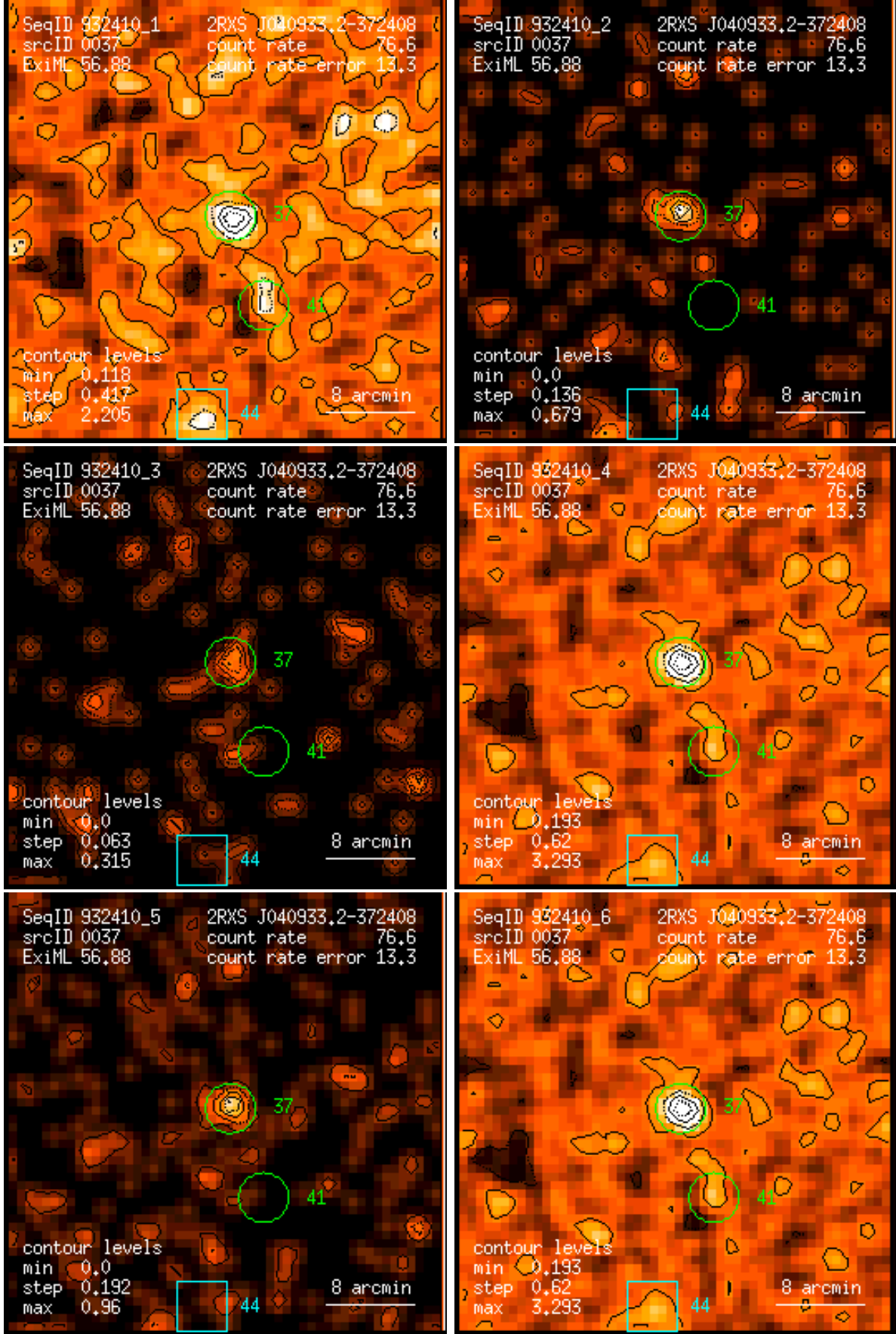
Figure 37: RASS 932410: detection 0037: band rate images, Gaussian filter: (1) PSPC channels 11 – 41, (2) 52 – 90, (3) 91 – 201, (4) 11 – 235, (5) 52 – 201, (6) 11 – 201. Broad band rates in counts/ks. Band rate contour levels in counts/ks/arcmin 2 .
