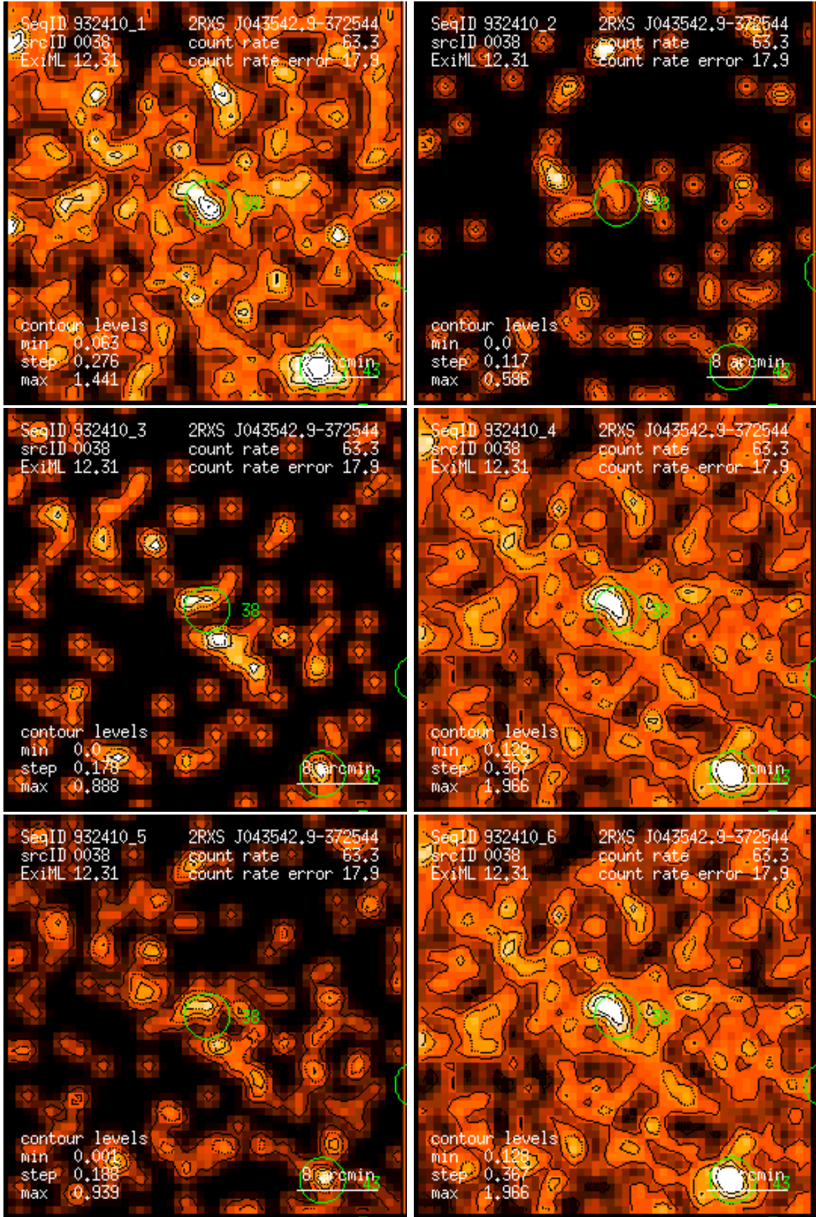
Figure 38: RASS 932410: detection 0038: band rate images, Gaussian filter: (1) PSPC channels 11 – 41, (2) 52 – 90, (3) 91 – 201, (4) 11 – 235, (5) 52 – 201, (6) 11 – 201. Broad band rates in counts/ks. Band rate contour levels in counts/ks/arcmin 2 .
