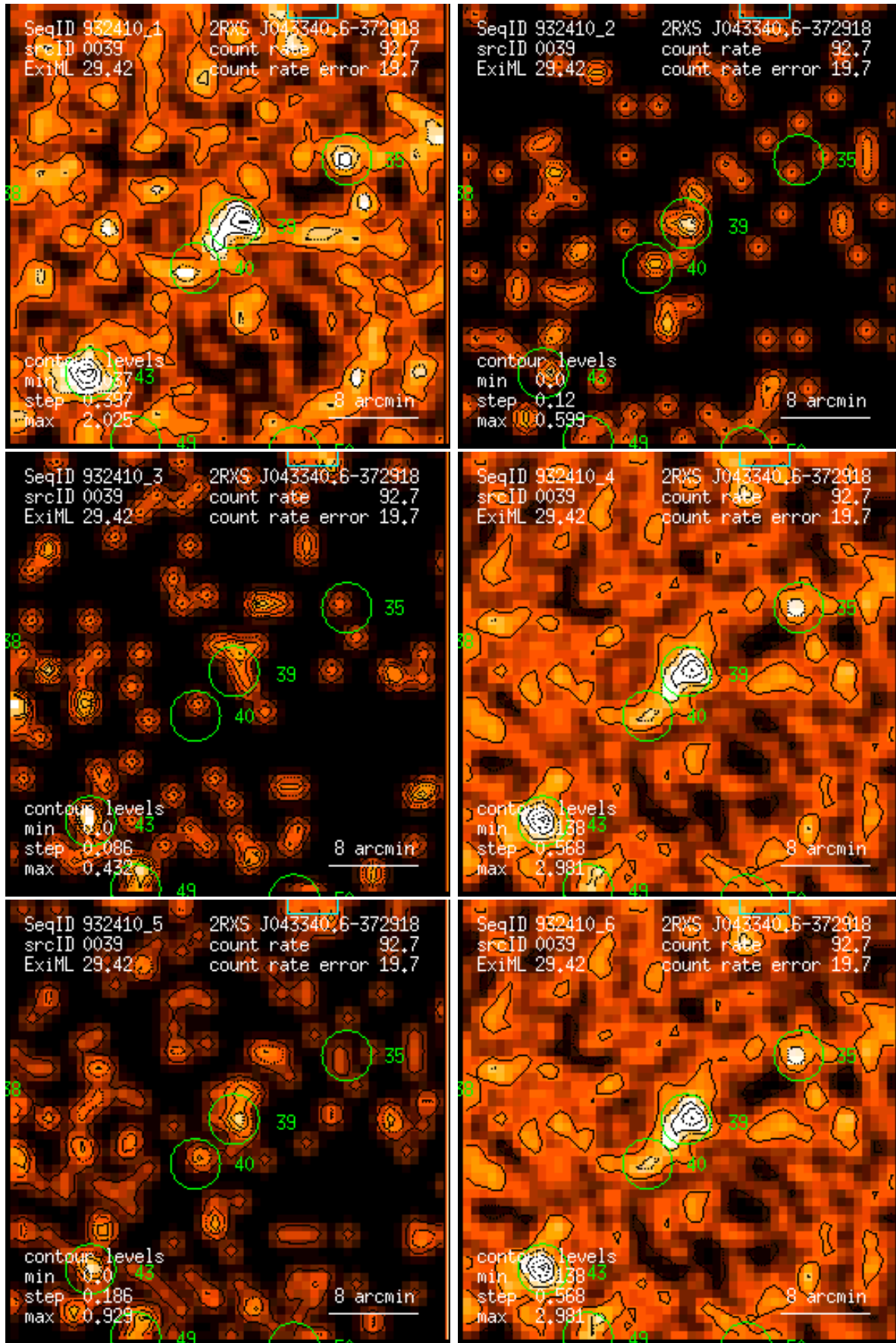
Figure 39: RASS 932410: detection 0039: band rate images, Gaussian filter: (1) PSPC channels 11 – 41, (2) 52 – 90, (3) 91 – 201, (4) 11 – 235, (5) 52 – 201, (6) 11 – 201. Broad band rates in counts/ks. Band rate contour levels in counts/ks/arcmin 2 .
