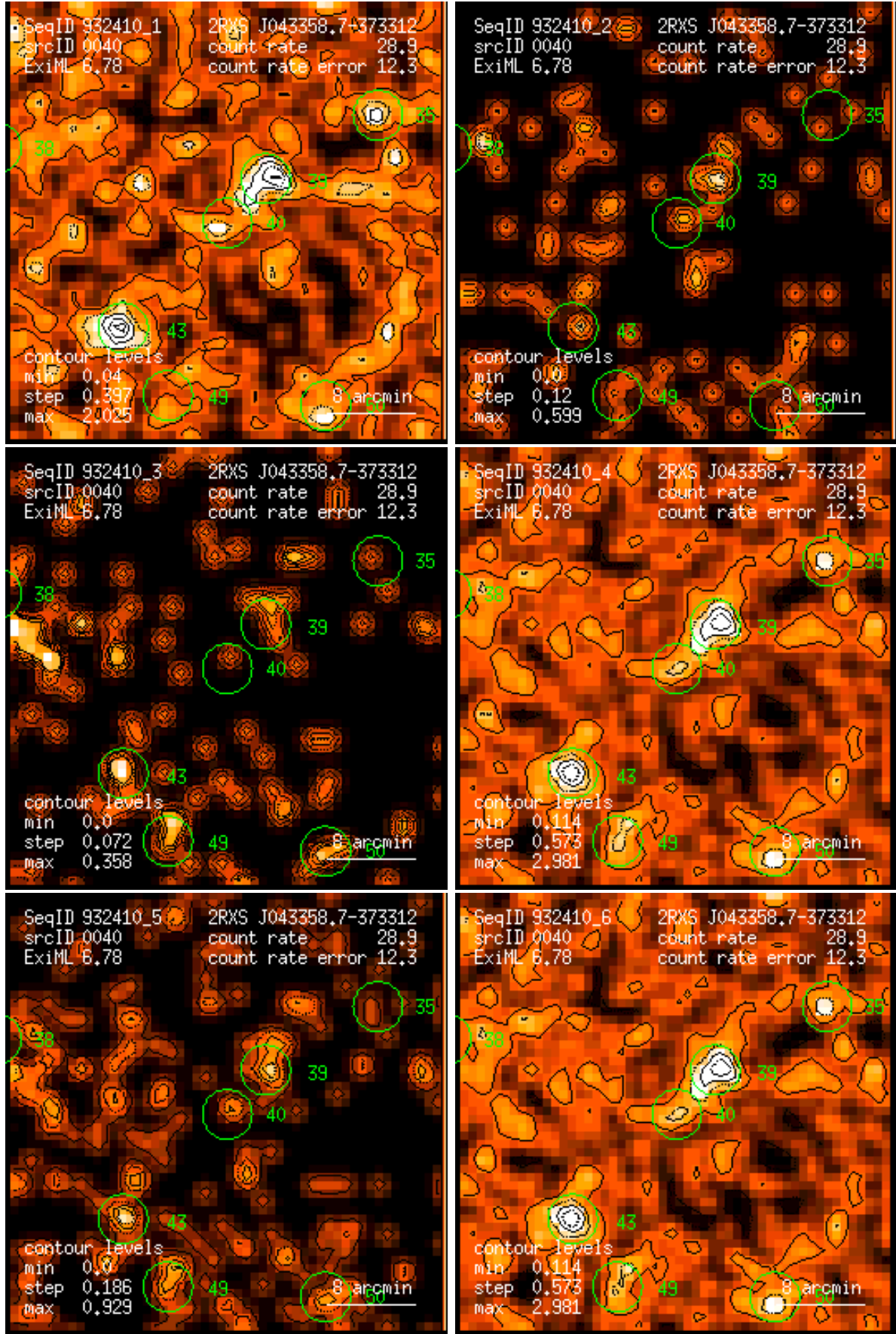
Figure 40: RASS 932410: detection 0040: band rate images, Gaussian filter: (1) PSPC channels 11 – 41, (2) 52 – 90, (3) 91 – 201, (4) 11 – 235, (5) 52 – 201, (6) 11 – 201. Broad band rates in counts/ks. Band rate contour levels in counts/ks/arcmin 2 .
