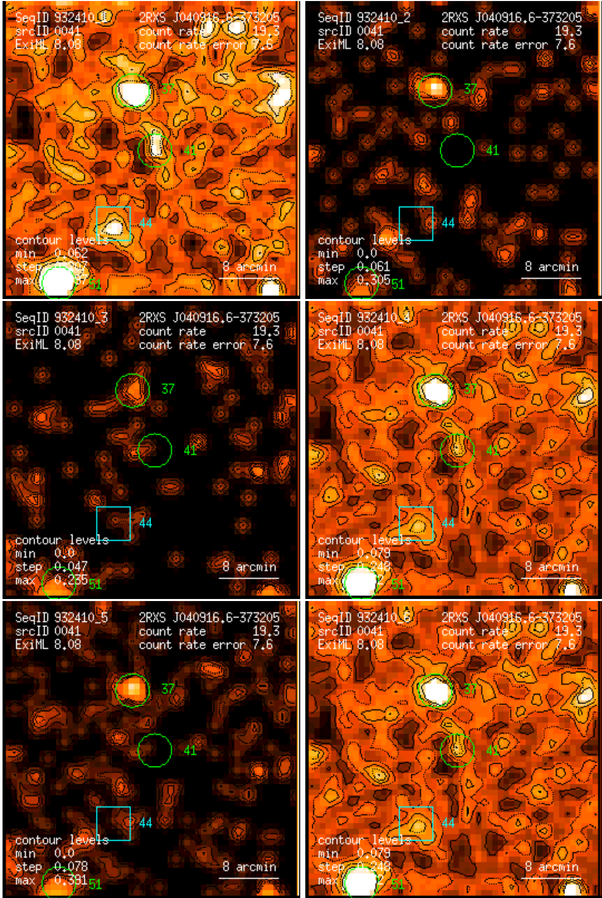
Figure 41: RASS 932410: detection 0041: band rate images, Gaussian filter: (1) PSPC channels 11 – 41, (2) 52 – 90, (3) 91 – 201, (4) 11 – 235, (5) 52 – 201, (6) 11 – 201. Broad band rates in counts/ks. Band rate contour levels in counts/ks/arcmin 2 .
