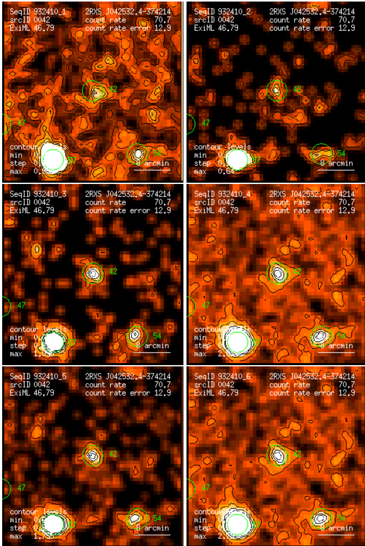
Figure 42: RASS 932410: detection 0042: band rate images, Gaussian filter: (1) PSPC channels 11 – 41, (2) 52 – 90, (3) 91 – 201, (4) 11 – 235, (5) 52 – 201, (6) 11 – 201. Broad band rates in counts/ks. Band rate contour levels in counts/ks/arcmin 2 .
