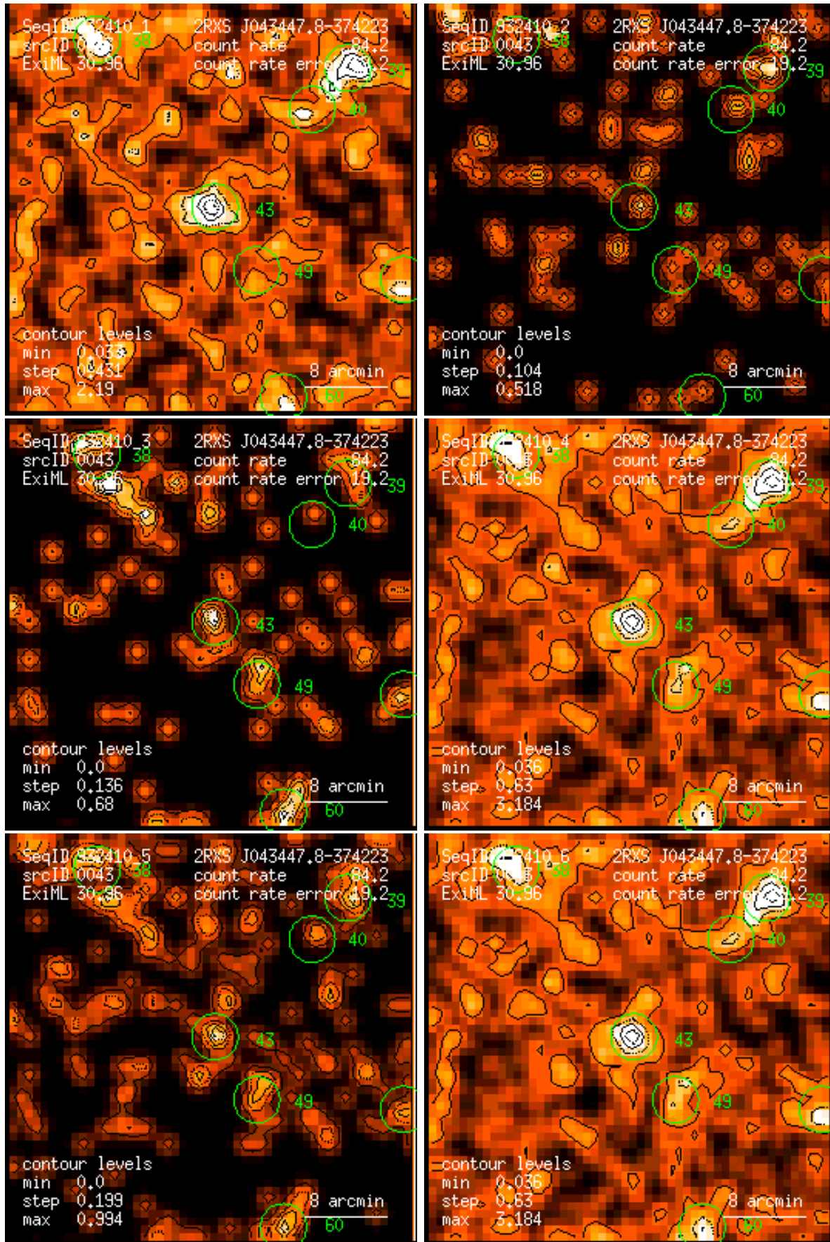
Figure 43: RASS 932410: detection 0043: band rate images, Gaussian filter: (1) PSPC channels 11 – 41, (2) 52 – 90, (3) 91 – 201, (4) 11 – 235, (5) 52 – 201, (6) 11 – 201. Broad band rates in counts/ks. Band rate contour levels in counts/ks/arcmin 2 .
