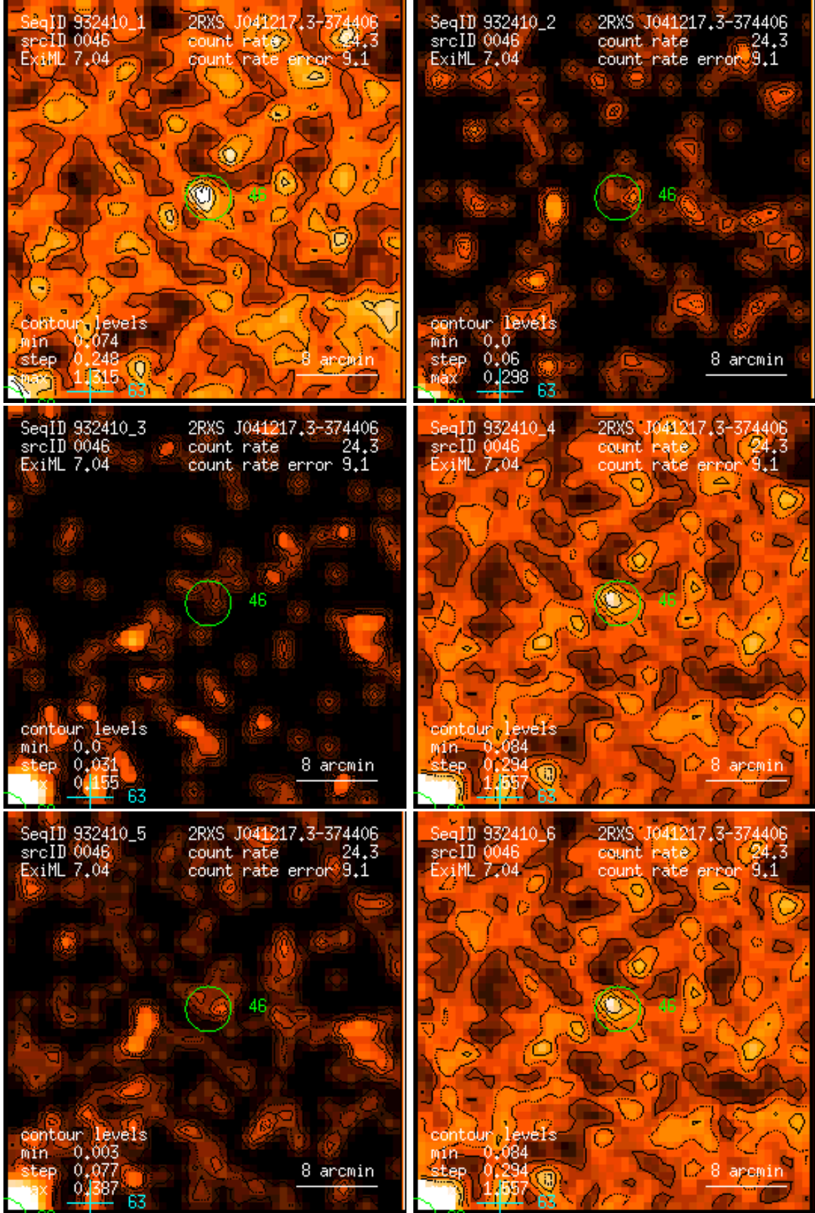
Figure 46: RASS 932410: detection 0046: band rate images, Gaussian filter: (1) PSPC channels 11 – 41, (2) 52 – 90, (3) 91 – 201, (4) 11 – 235, (5) 52 – 201, (6) 11 – 201. Broad band rates in counts/ks. Band rate contour levels in counts/ks/arcmin 2 .
