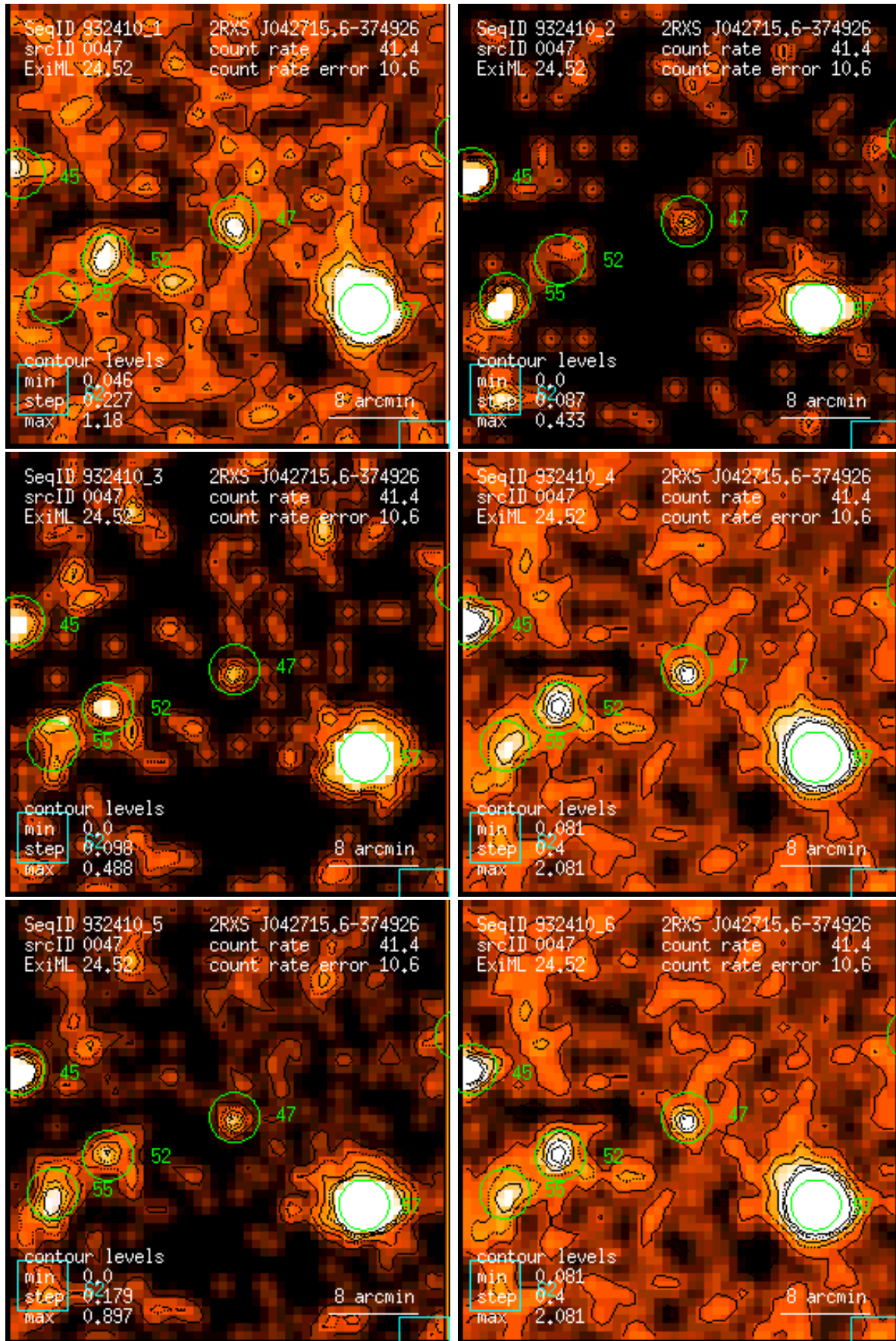
Figure 47: RASS 932410: detection 0047: band rate images, Gaussian filter: (1) PSPC channels 11 – 41, (2) 52 – 90, (3) 91 – 201, (4) 11 – 235, (5) 52 – 201, (6) 11 – 201. Broad band rates in counts/ks. Band rate contour levels in counts/ks/arcmin 2 .
