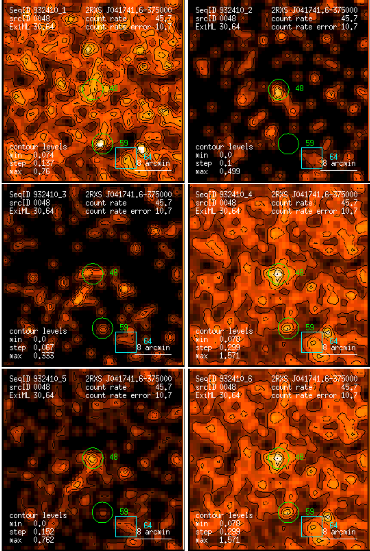
Figure 48: RASS 932410: detection 0048: band rate images, Gaussian filter: (1) PSPC channels 11 – 41, (2) 52 – 90, (3) 91 – 201, (4) 11 – 235, (5) 52 – 201, (6) 11 – 201. Broad band rates in counts/ks. Band rate contour levels in counts/ks/arcmin 2 .
