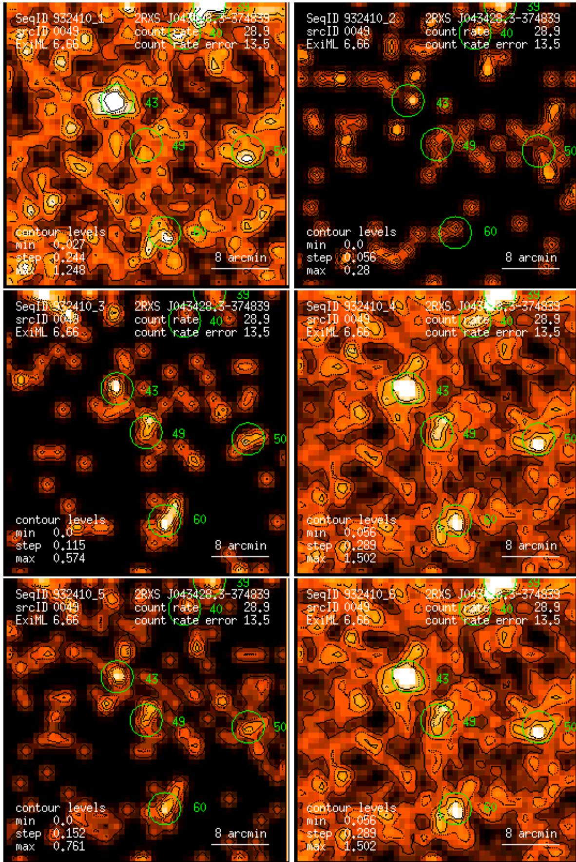
Figure 49: RASS 932410: detection 0049: band rate images, Gaussian filter: (1) PSPC channels 11 – 41, (2) 52 – 90, (3) 91 – 201, (4) 11 – 235, (5) 52 – 201, (6) 11 – 201. Broad band rates in counts/ks. Band rate contour levels in counts/ks/arcmin 2 .
