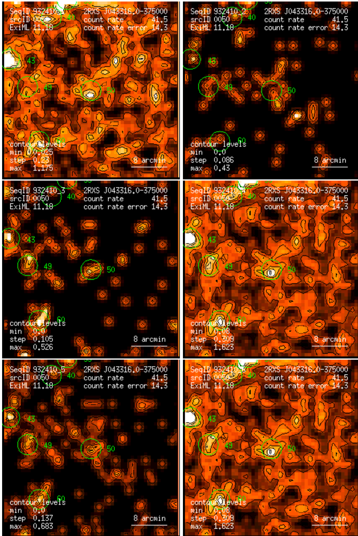
Figure 50: RASS 932410: detection 0050: band rate images, Gaussian filter: (1) PSPC channels 11 – 41, (2) 52 – 90, (3) 91 – 201, (4) 11 – 235, (5) 52 – 201, (6) 11 – 201. Broad band rates in counts/ks. Band rate contour levels in counts/ks/arcmin 2 .
