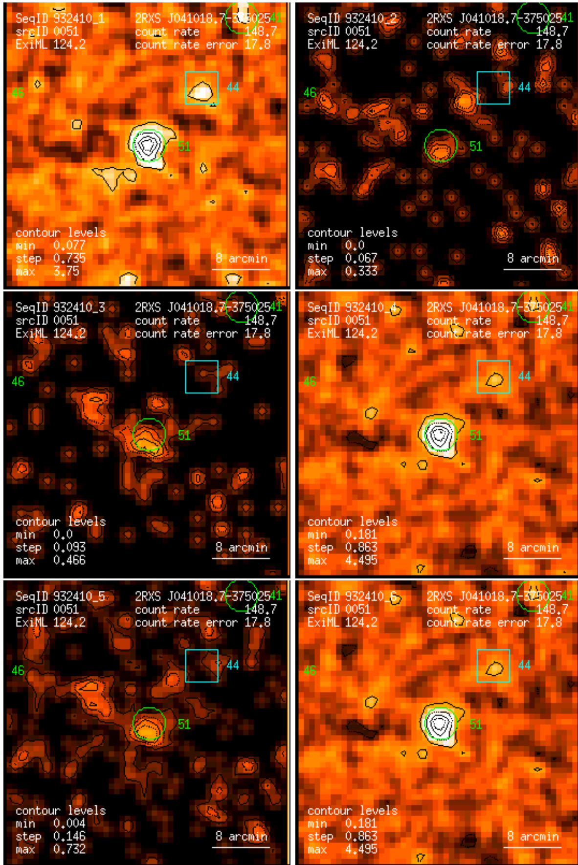
Figure 51: RASS 932410: detection 0051: band rate images, Gaussian filter: (1) PSPC channels 11 – 41, (2) 52 – 90, (3) 91 – 201, (4) 11 – 235, (5) 52 – 201, (6) 11 – 201. Broad band rates in counts/ks. Band rate contour levels in counts/ks/arcmin 2 .
