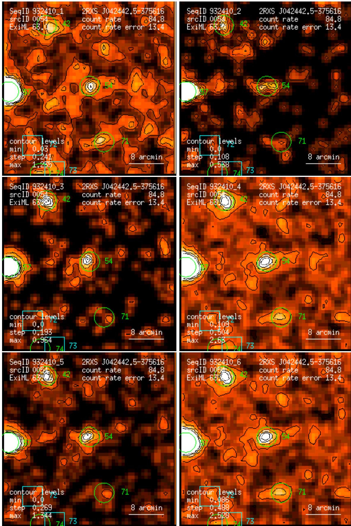
Figure 54: RASS 932410: detection 0054: band rate images, Gaussian filter: (1) PSPC channels 11 – 41, (2) 52 – 90, (3) 91 – 201, (4) 11 – 235, (5) 52 – 201, (6) 11 – 201. Broad band rates in counts/ks. Band rate contour levels in counts/ks/arcmin 2 .
