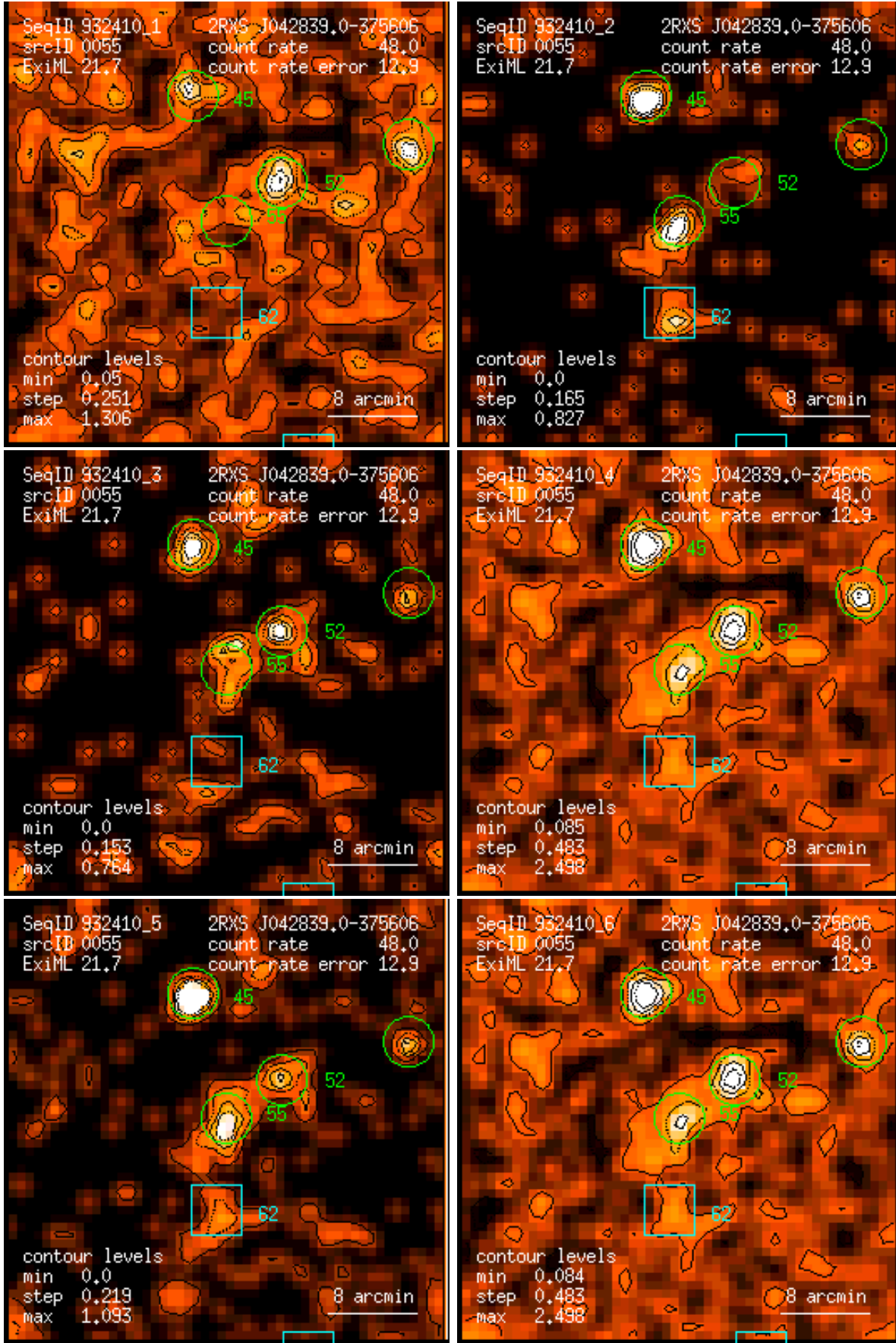
Figure 55: RASS 932410: detection 0055: band rate images, Gaussian filter: (1) PSPC channels 11 – 41, (2) 52 – 90, (3) 91 – 201, (4) 11 – 235, (5) 52 – 201, (6) 11 – 201. Broad band rates in counts/ks. Band rate contour levels in counts/ks/arcmin 2 .
