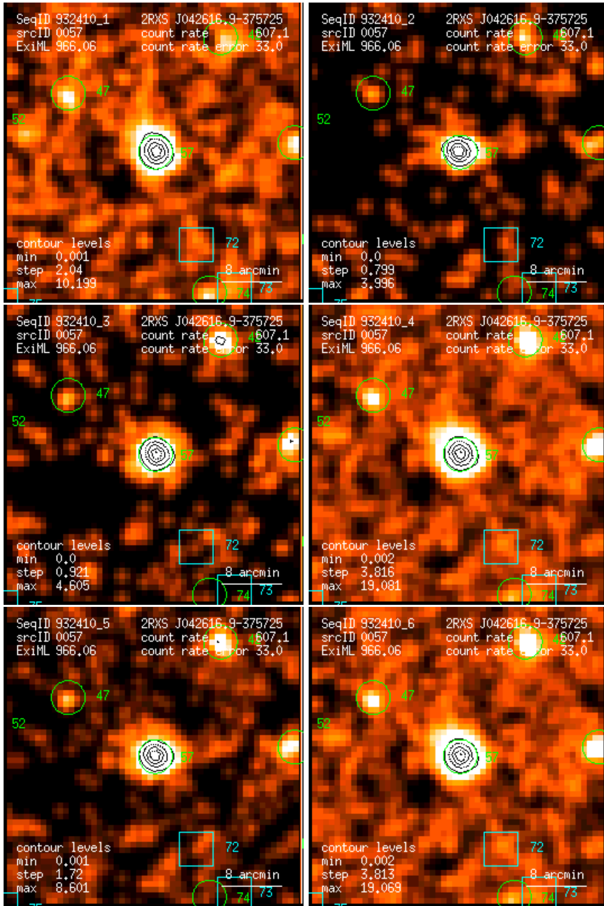
Figure 57: RASS 932410: detection 0057: band rate images, Gaussian filter: (1) PSPC channels 11 – 41, (2) 52 – 90, (3) 91 – 201, (4) 11 – 235, (5) 52 – 201, (6) 11 – 201. Broad band rates in counts/ks. Band rate contour levels in counts/ks/arcmin 2 .
