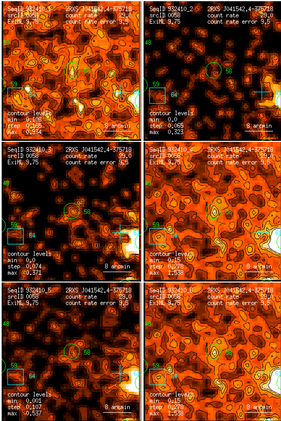
Figure 58: RASS 932410: detection 0058: band rate images, Gaussian filter: (1) PSPC channels 11 – 41, (2) 52 – 90, (3) 91 – 201, (4) 11 – 235, (5) 52 – 201, (6) 11 – 201. Broad band rates in counts/ks. Band rate contour levels in counts/ks/arcmin 2 .
