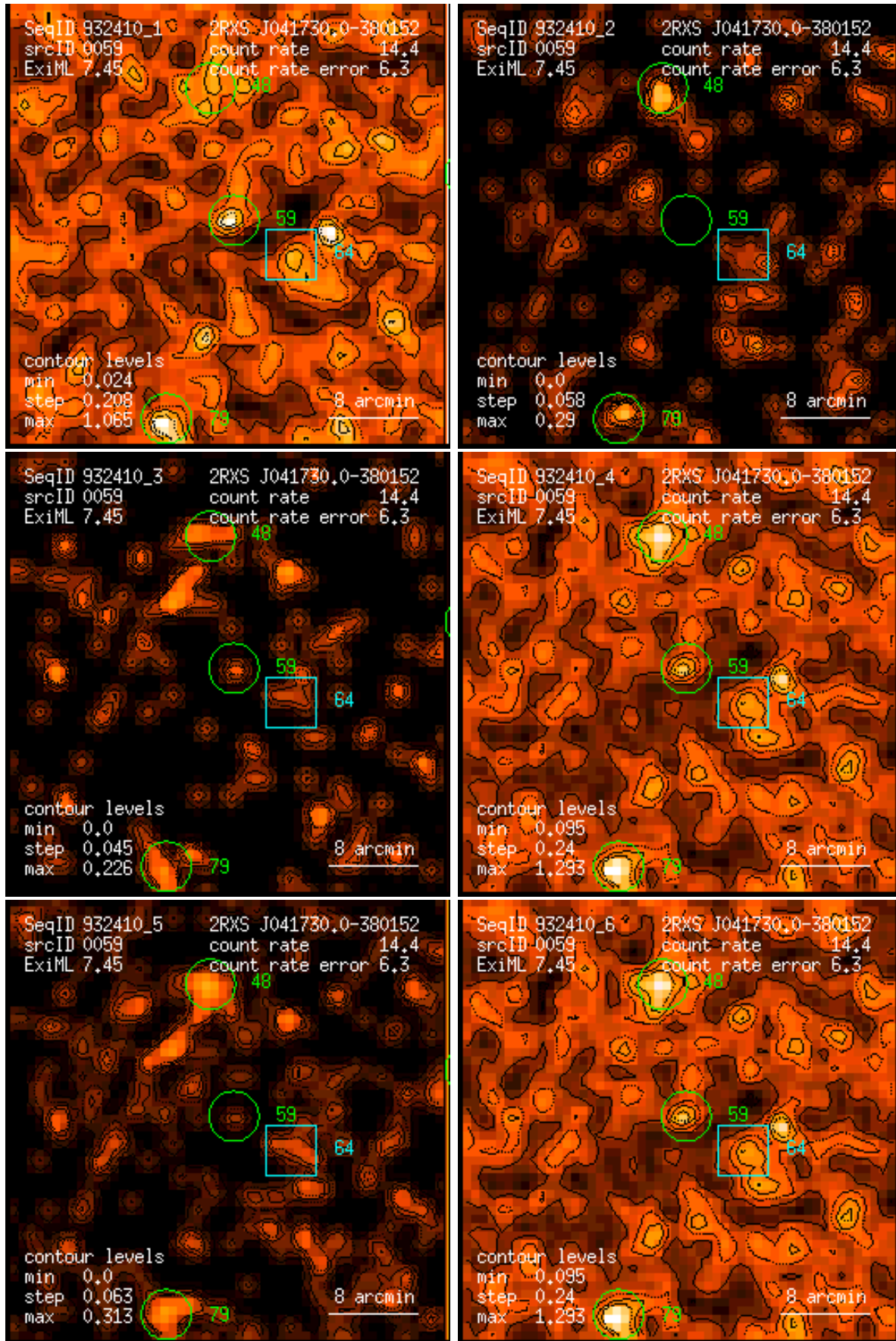
Figure 59: RASS 932410: detection 0059: band rate images, Gaussian filter: (1) PSPC channels 11 – 41, (2) 52 – 90, (3) 91 – 201, (4) 11 – 235, (5) 52 – 201, (6) 11 – 201. Broad band rates in counts/ks. Band rate contour levels in counts/ks/arcmin 2 .
