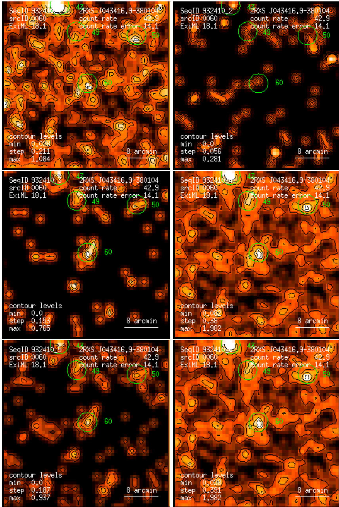
Figure 60: RASS 932410: detection 0060: band rate images, Gaussian filter: (1) PSPC channels 11 – 41, (2) 52 – 90, (3) 91 – 201, (4) 11 – 235, (5) 52 – 201, (6) 11 – 201. Broad band rates in counts/ks. Band rate contour levels in counts/ks/arcmin 2 .
