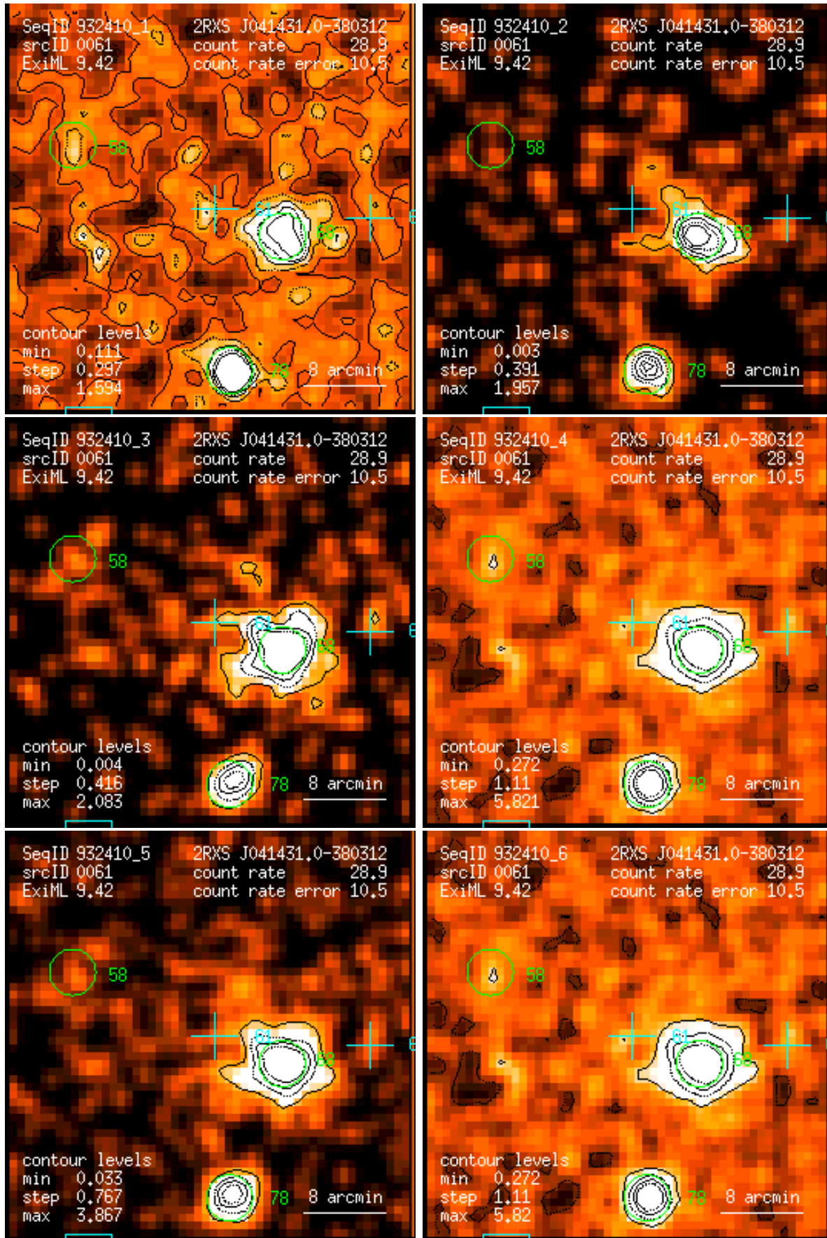
Figure 61: RASS 932410: detection 0061: band rate images, Gaussian filter: (1) PSPC channels 11 – 41, (2) 52 – 90, (3) 91 – 201, (4) 11 – 235, (5) 52 – 201, (6) 11 – 201. Broad band rates in counts/ks. Band rate contour levels in counts/ks/arcmin 2 .
