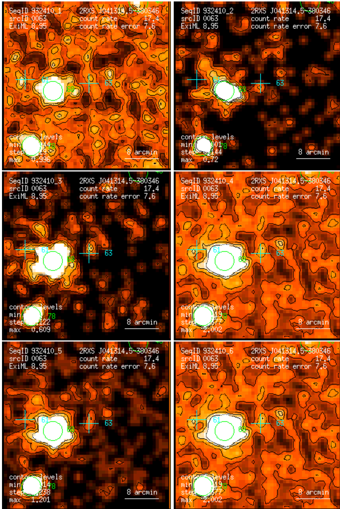
Figure 63: RASS 932410: detection 0063: band rate images, Gaussian filter: (1) PSPC channels 11 – 41, (2) 52 – 90, (3) 91 – 201, (4) 11 – 235, (5) 52 – 201, (6) 11 – 201. Broad band rates in counts/ks. Band rate contour levels in counts/ks/arcmin 2 .
