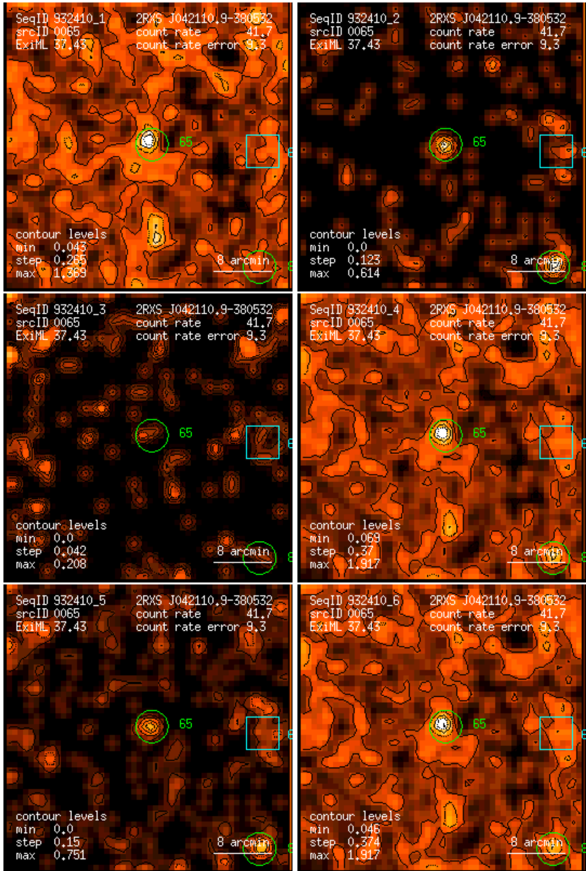
Figure 65: RASS 932410: detection 0065: band rate images, Gaussian filter: (1) PSPC channels 11 – 41, (2) 52 – 90, (3) 91 – 201, (4) 11 – 235, (5) 52 – 201, (6) 11 – 201. Broad band rates in counts/ks. Band rate contour levels in counts/ks/arcmin 2 .
