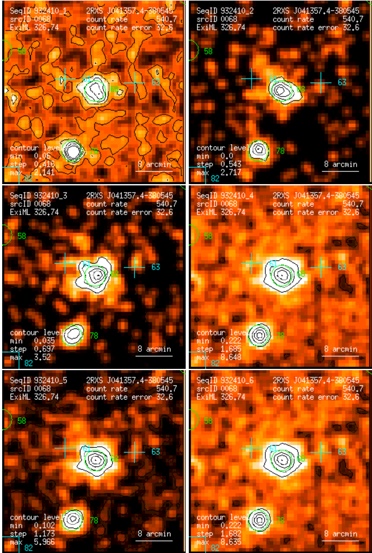
Figure 68: RASS 932410: detection 0068: band rate images, Gaussian filter: (1) PSPC channels 11 – 41, (2) 52 – 90, (3) 91 – 201, (4) 11 – 235, (5) 52 – 201, (6) 11 – 201. Broad band rates in counts/ks. Band rate contour levels in counts/ks/arcmin 2 .
