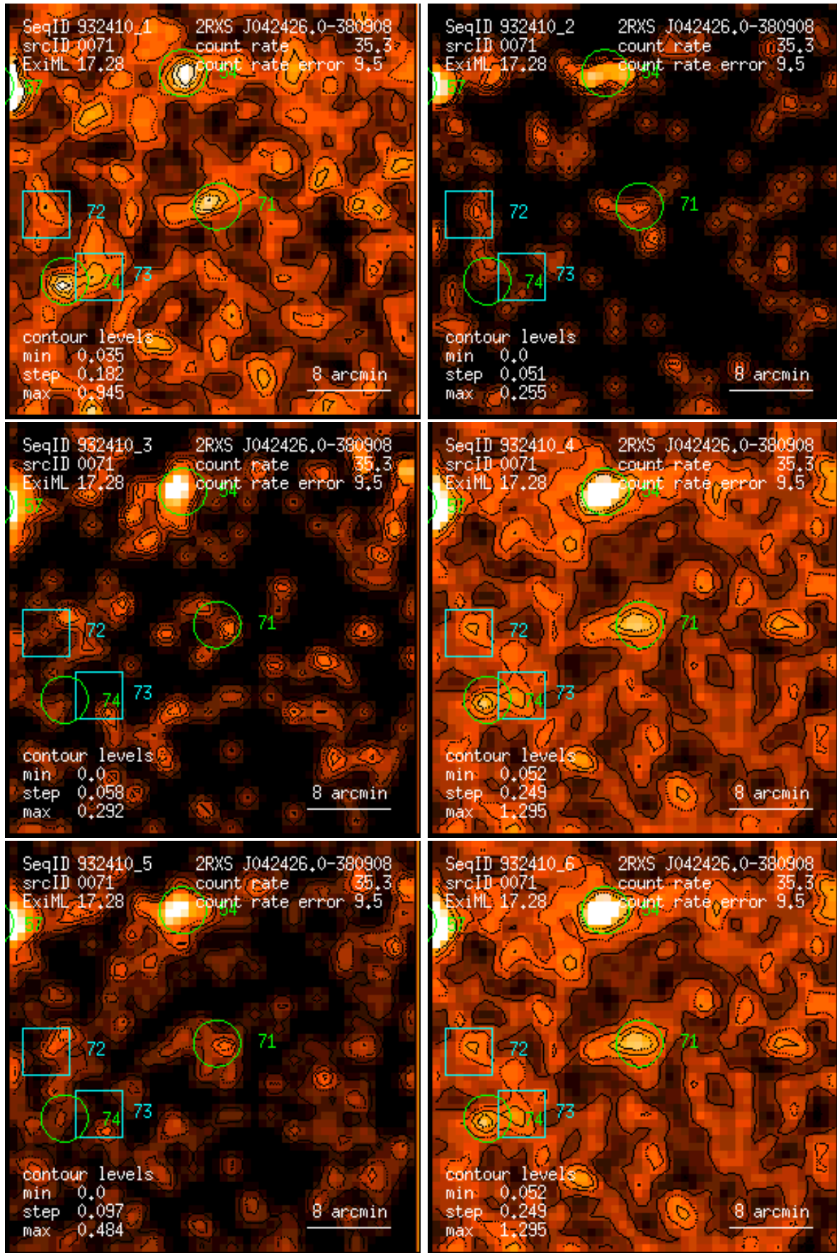
Figure 71: RASS 932410: detection 0071: band rate images, Gaussian filter: (1) PSPC channels 11 – 41, (2) 52 – 90, (3) 91 – 201, (4) 11 – 235, (5) 52 – 201, (6) 11 – 201. Broad band rates in counts/ks. Band rate contour levels in counts/ks/arcmin 2 .
