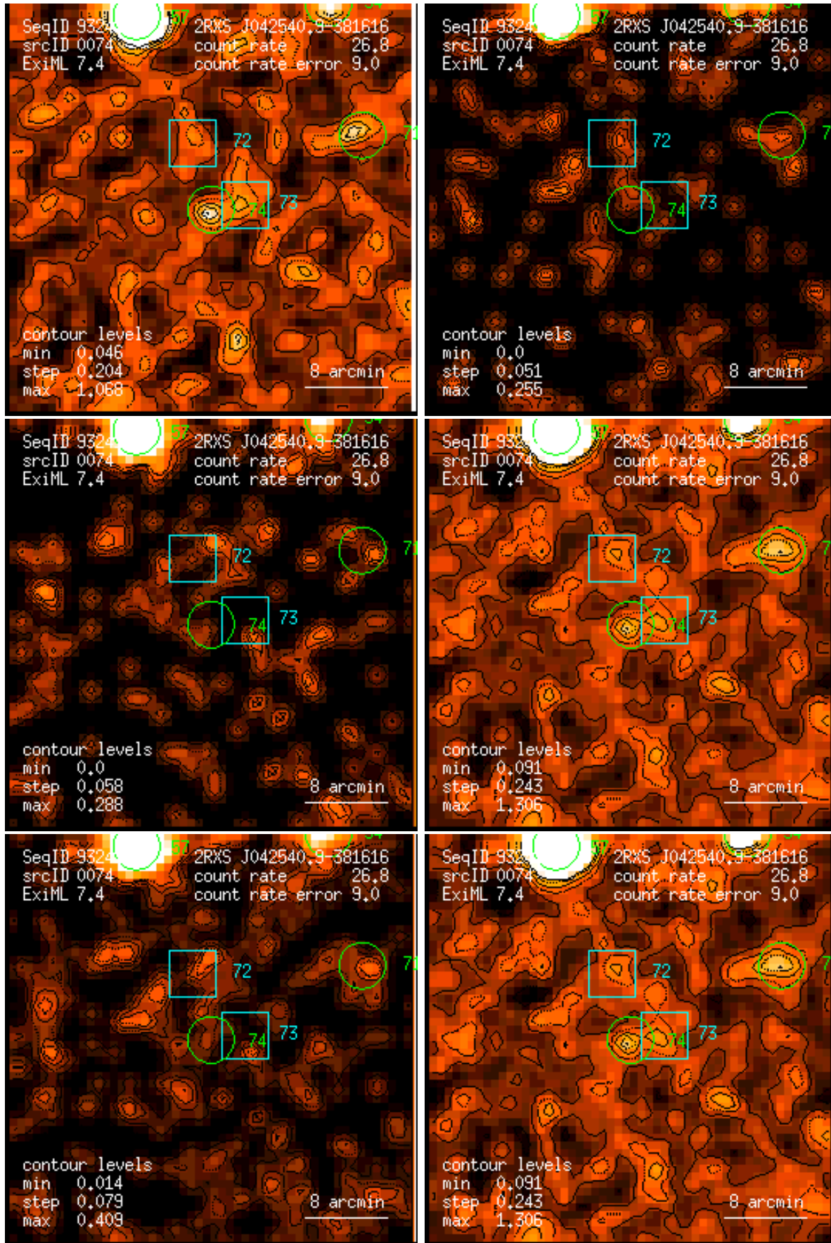
Figure 74: RASS 932410: detection 0074: band rate images, Gaussian filter: (1) PSPC channels 11 – 41, (2) 52 – 90, (3) 91 – 201, (4) 11 – 235, (5) 52 – 201, (6) 11 – 201. Broad band rates in counts/ks. Band rate contour levels in counts/ks/arcmin 2 .
