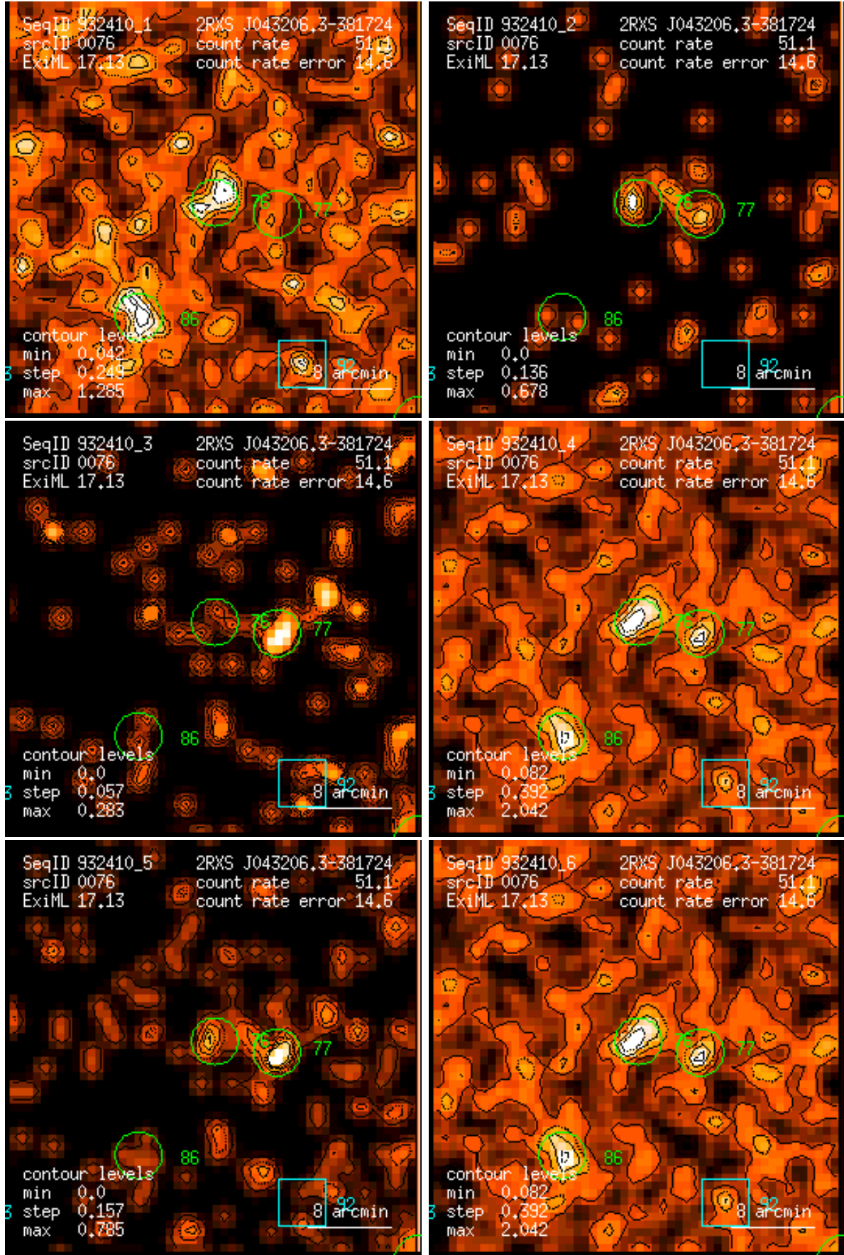
Figure 76: RASS 932410: detection 0076: band rate images, Gaussian filter: (1) PSPC channels 11 – 41, (2) 52 – 90, (3) 91 – 201, (4) 11 – 235, (5) 52 – 201, (6) 11 – 201. Broad band rates in counts/ks. Band rate contour levels in counts/ks/arcmin 2 .
