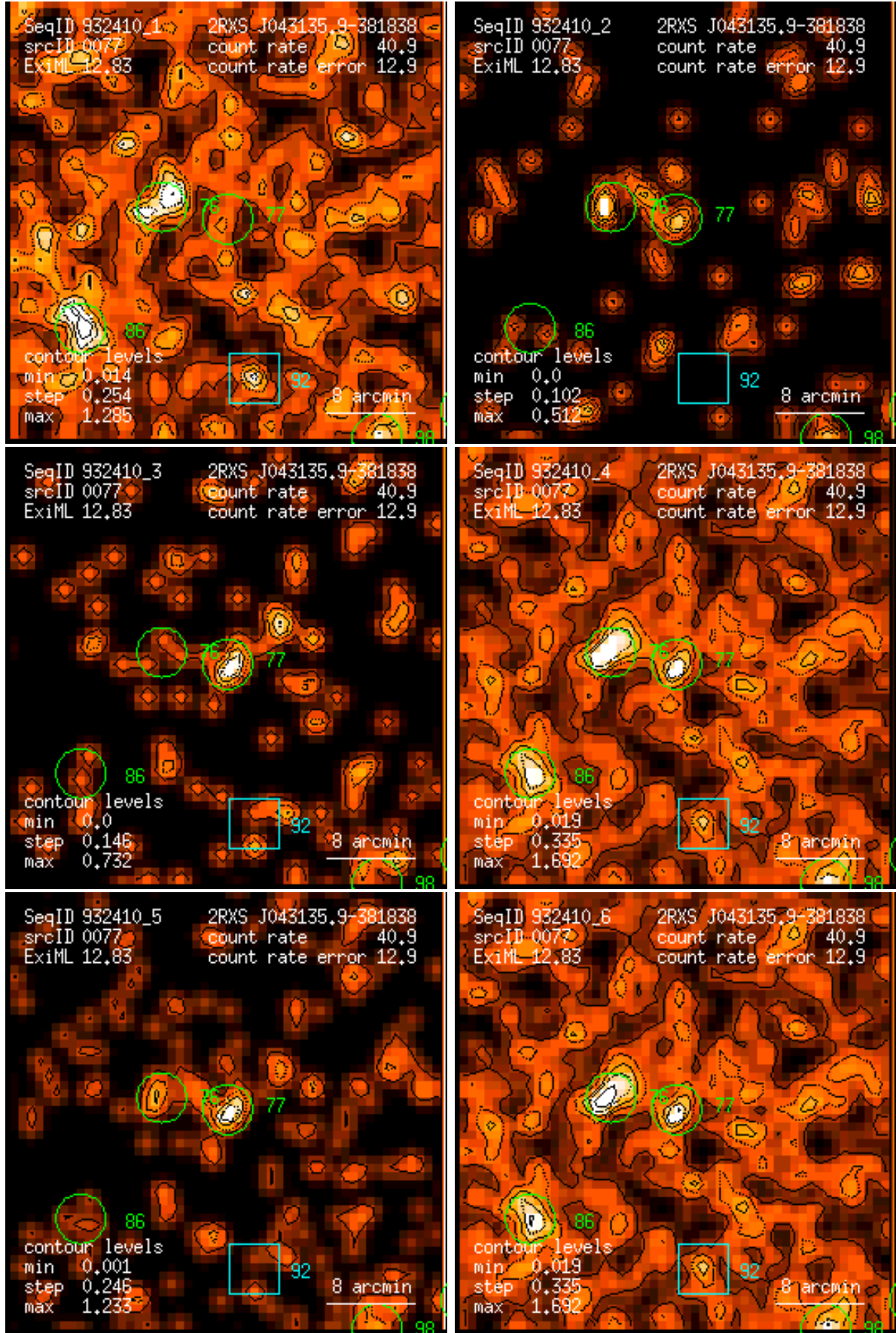
Figure 77: RASS 932410: detection 0077: band rate images, Gaussian filter: (1) PSPC channels 11 – 41, (2) 52 – 90, (3) 91 – 201, (4) 11 – 235, (5) 52 – 201, (6) 11 – 201. Broad band rates in counts/ks. Band rate contour levels in counts/ks/arcmin 2 .
