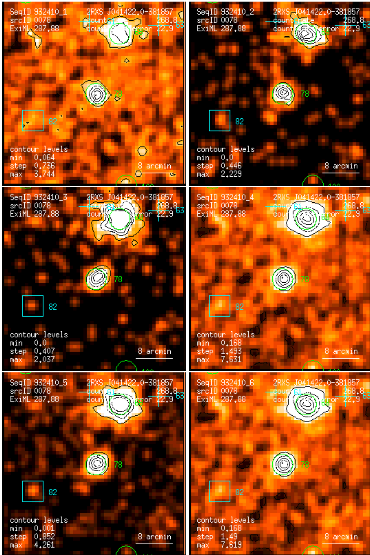
Figure 78: RASS 932410: detection 0078: band rate images, Gaussian filter: (1) PSPC channels 11 – 41, (2) 52 – 90, (3) 91 – 201, (4) 11 – 235, (5) 52 – 201, (6) 11 – 201. Broad band rates in counts/ks. Band rate contour levels in counts/ks/arcmin 2 .
