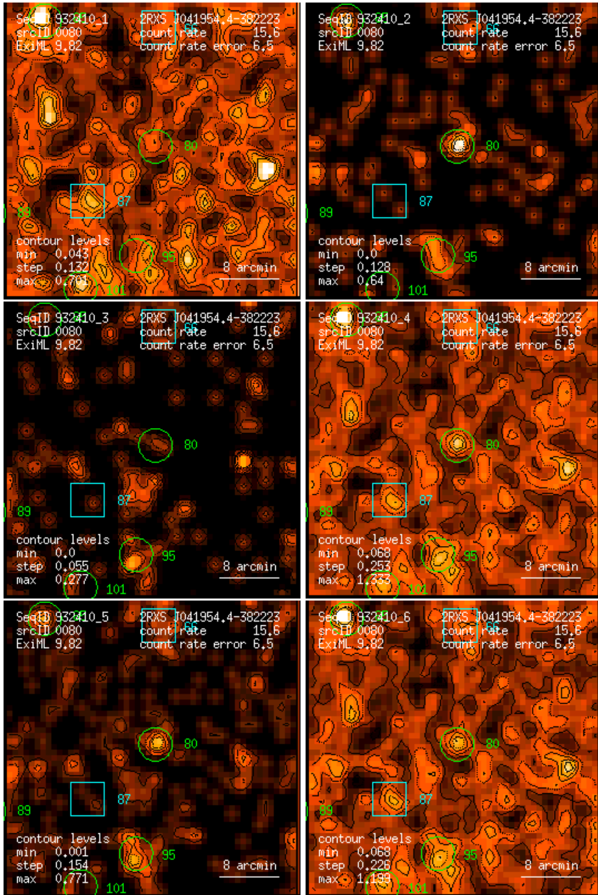
Figure 80: RASS 932410: detection 0080: band rate images, Gaussian filter: (1) PSPC channels 11 – 41, (2) 52 – 90, (3) 91 – 201, (4) 11 – 235, (5) 52 – 201, (6) 11 – 201. Broad band rates in counts/ks. Band rate contour levels in counts/ks/arcmin 2 .
