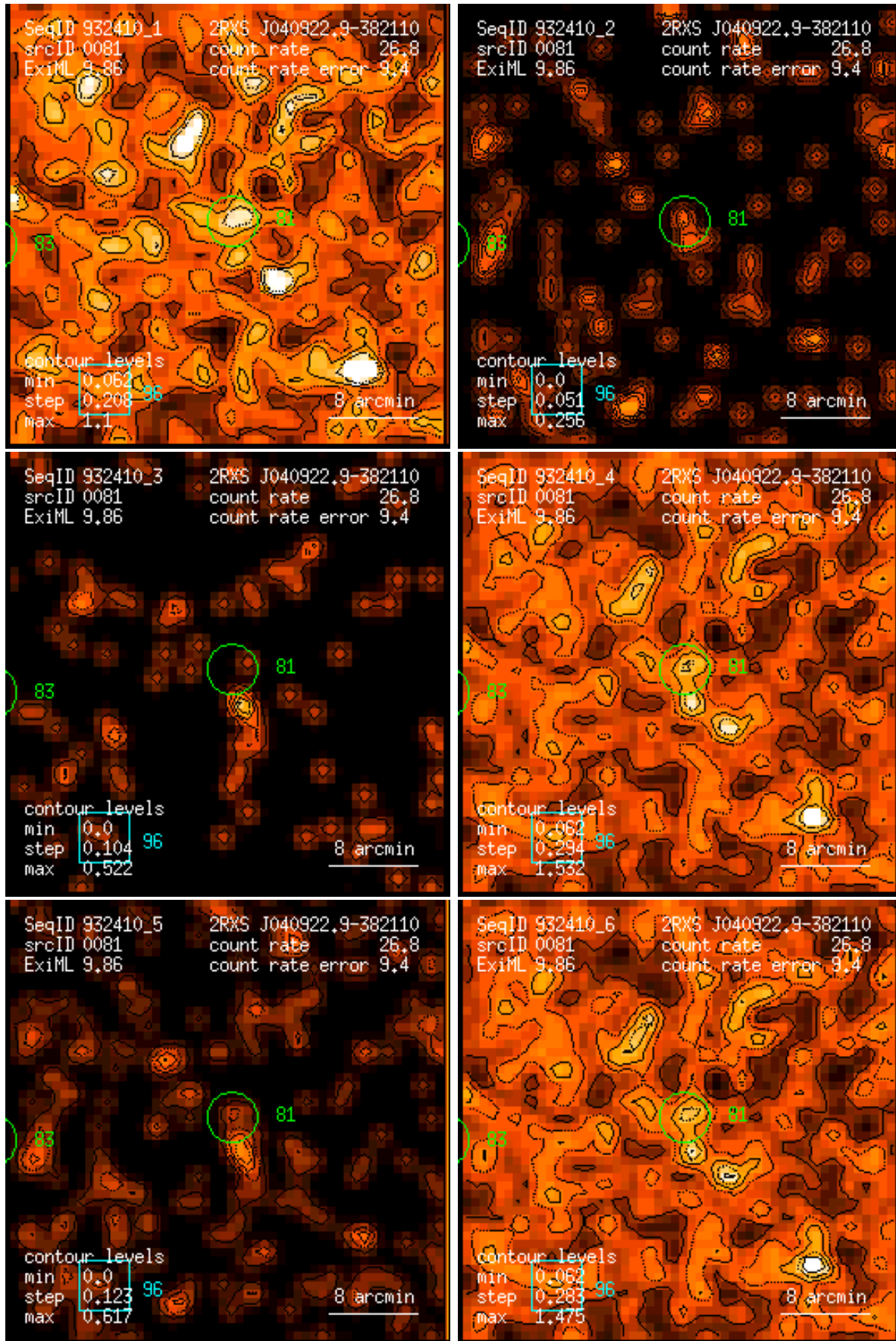
Figure 81: RASS 932410: detection 0081: band rate images, Gaussian filter: (1) PSPC channels 11 – 41, (2) 52 – 90, (3) 91 – 201, (4) 11 – 235, (5) 52 – 201, (6) 11 – 201. Broad band rates in counts/ks. Band rate contour levels in counts/ks/arcmin 2 .
