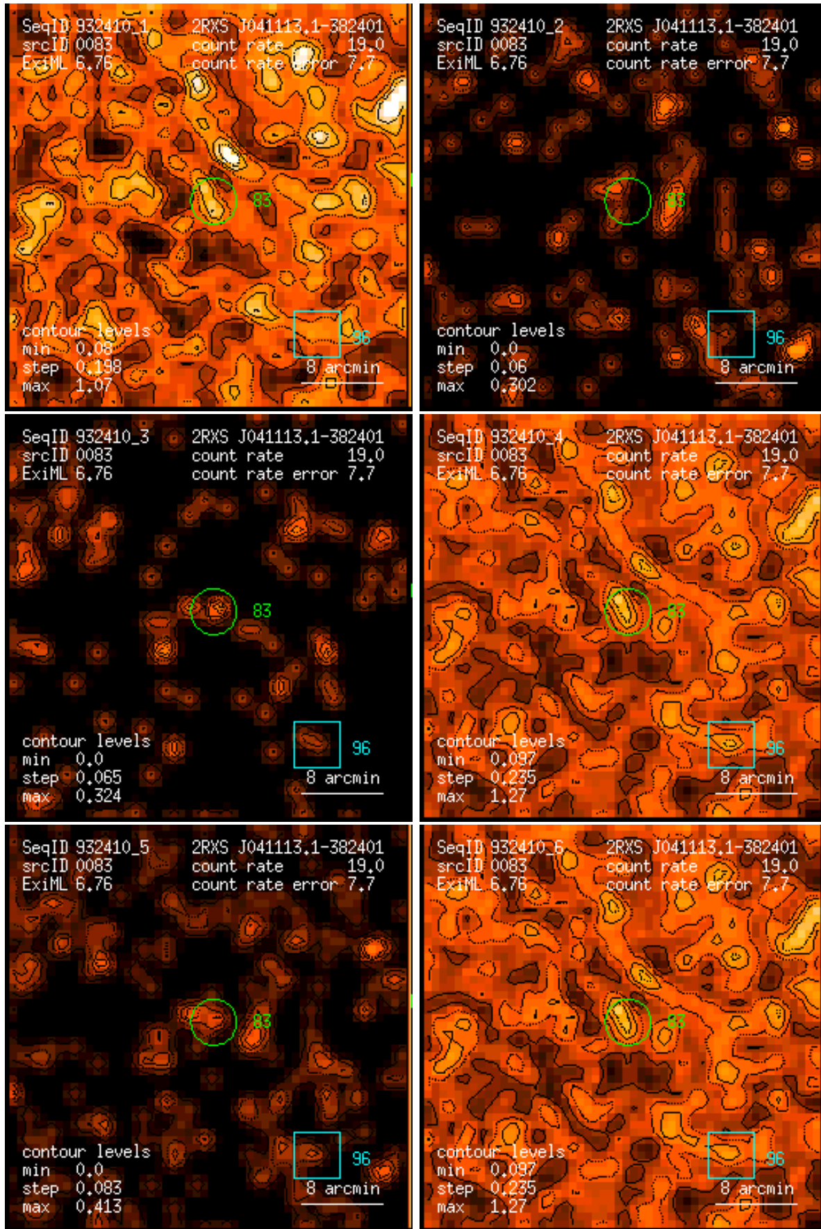
Figure 83: RASS 932410: detection 0083: band rate images, Gaussian filter: (1) PSPC channels 11 – 41, (2) 52 – 90, (3) 91 – 201, (4) 11 – 235, (5) 52 – 201, (6) 11 – 201. Broad band rates in counts/ks. Band rate contour levels in counts/ks/arcmin 2 .
