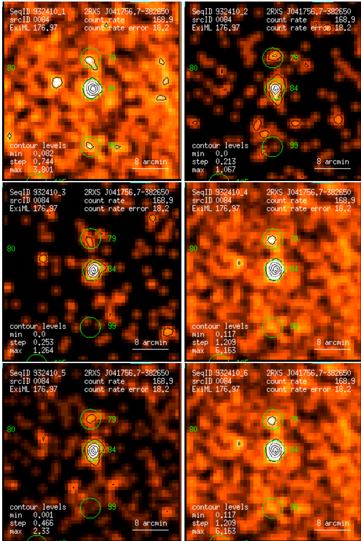
Figure 84: RASS 932410: detection 0084: band rate images, Gaussian filter: (1) PSPC channels 11 – 41, (2) 52 – 90, (3) 91 – 201, (4) 11 – 235, (5) 52 – 201, (6) 11 – 201. Broad band rates in counts/ks. Band rate contour levels in counts/ks/arcmin 2 .
