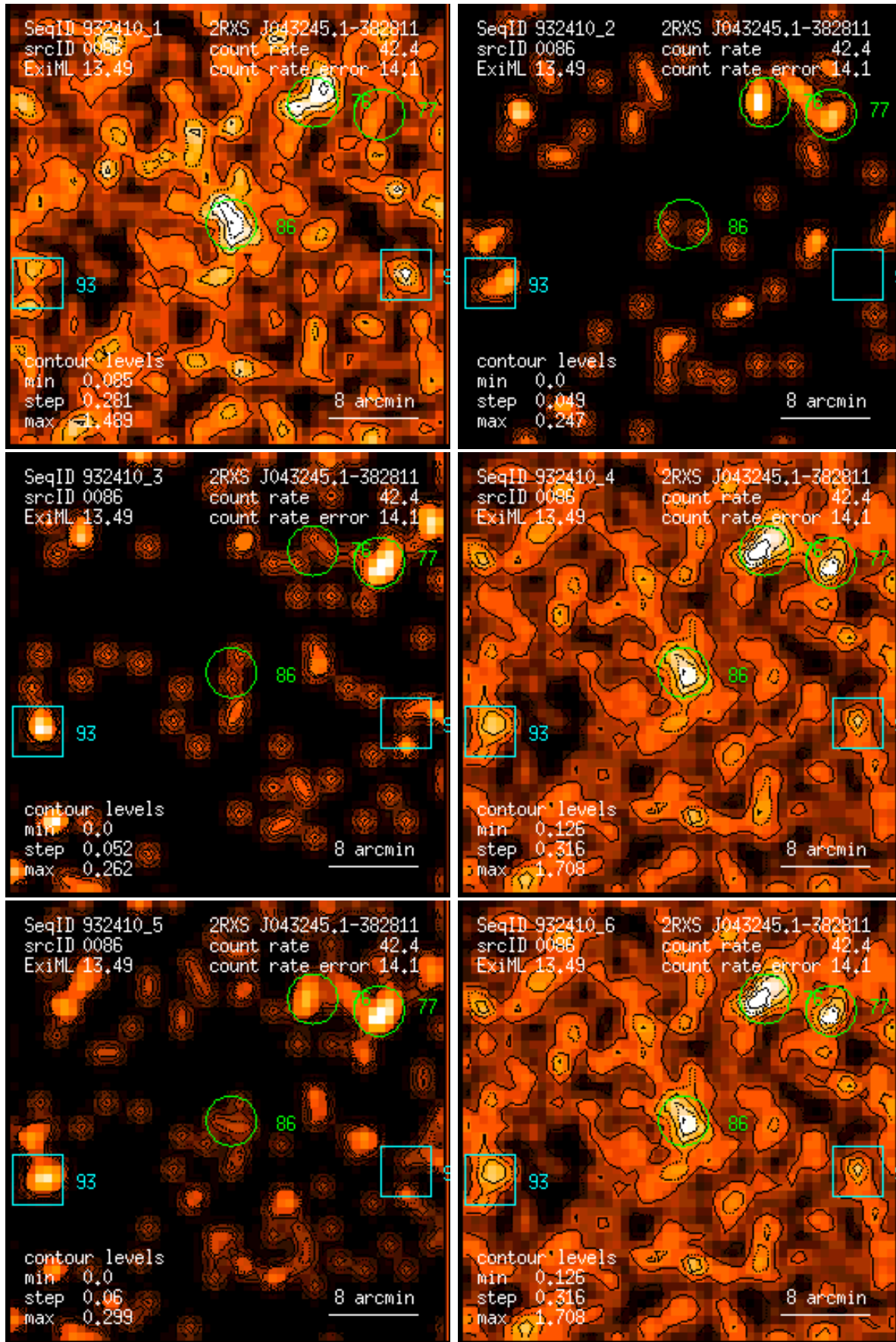
Figure 86: RASS 932410: detection 0086: band rate images, Gaussian filter: (1) PSPC channels 11 – 41, (2) 52 – 90, (3) 91 – 201, (4) 11 – 235, (5) 52 – 201, (6) 11 – 201. Broad band rates in counts/ks. Band rate contour levels in counts/ks/arcmin 2 .
