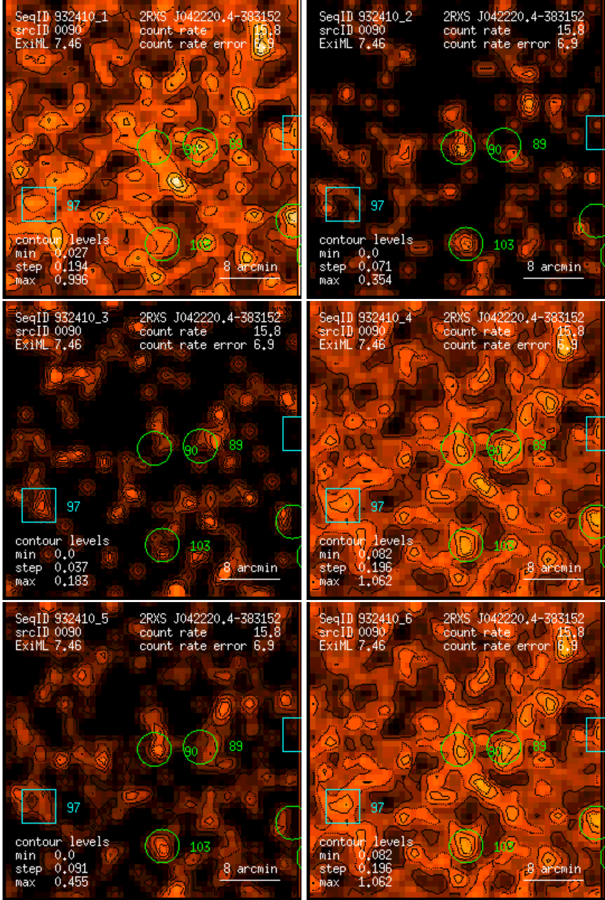
Figure 90: RASS 932410: detection 0090: band rate images, Gaussian filter: (1) PSPC channels 11 – 41, (2) 52 – 90, (3) 91 – 201, (4) 11 – 235, (5) 52 – 201, (6) 11 – 201. Broad band rates in counts/ks. Band rate contour levels in counts/ks/arcmin 2 .
