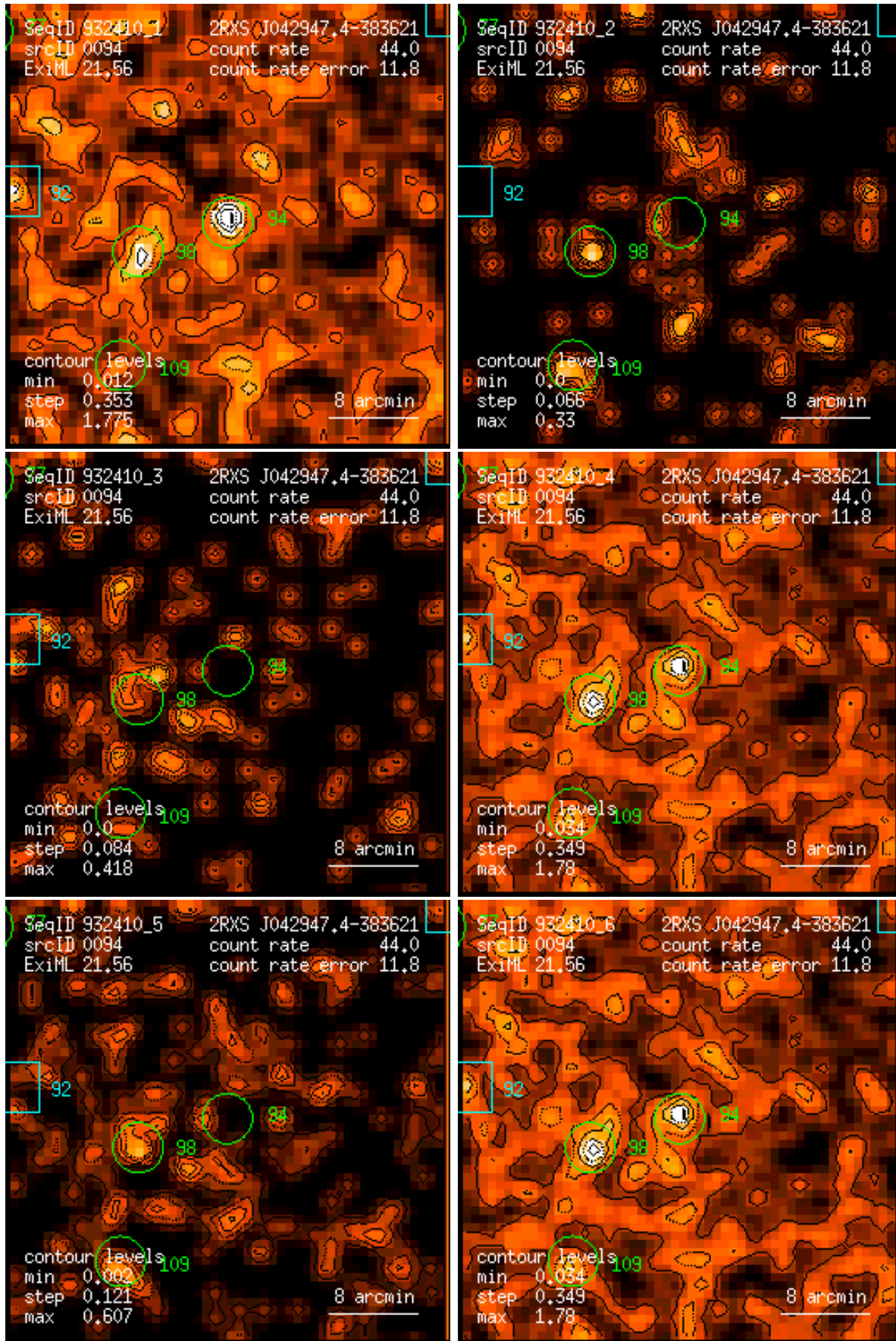
Figure 94: RASS 932410: detection 0094: band rate images, Gaussian filter: (1) PSPC channels 11 – 41, (2) 52 – 90, (3) 91 – 201, (4) 11 – 235, (5) 52 – 201, (6) 11 – 201. Broad band rates in counts/ks. Band rate contour levels in counts/ks/arcmin 2 .
